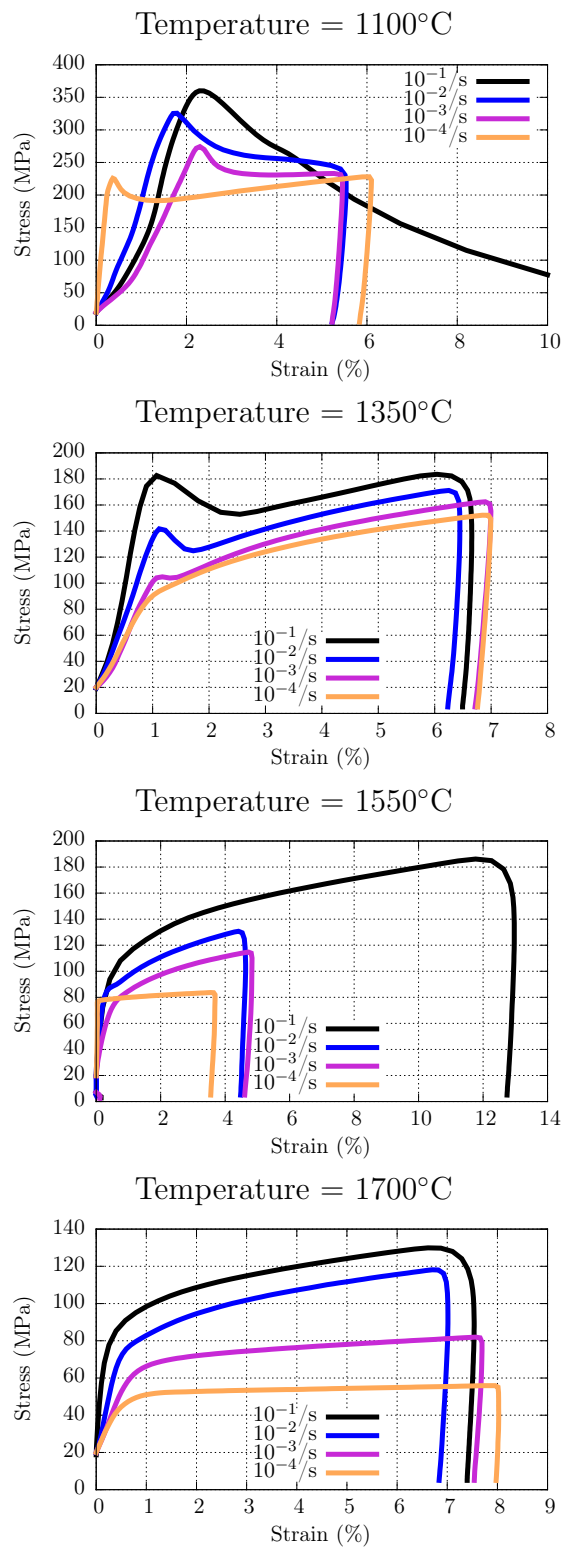
Figure 4: Stress - true strain curves obtained at different temperatures.
