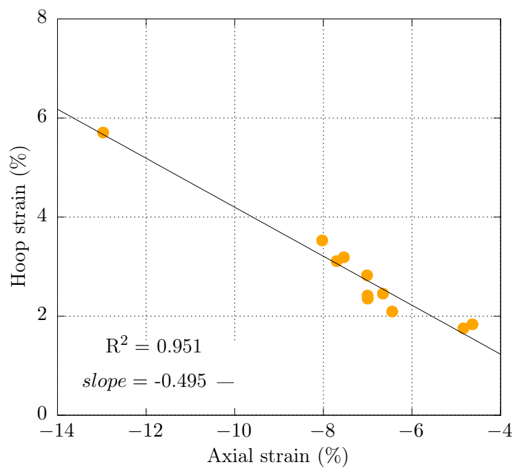
Figure 6: Average residual hoop strains versus residual axial strains (all tests except at 1100°C).
