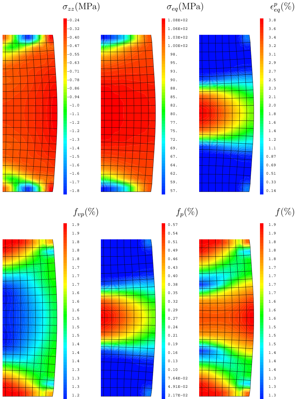
Figure 18: Isovalues of axial ( \sigma_{zz} ) and equivalent ( \sigma_{eq} ) stresses, equivalent plastic strain ( \epsilon_{eq}^p ), viscoplastic porosity ( f_{vp} , no GB cracking), plastic porosity ( f_p ), total porosity ( f ) during the test at 1550°C and 10 -1 /s.
