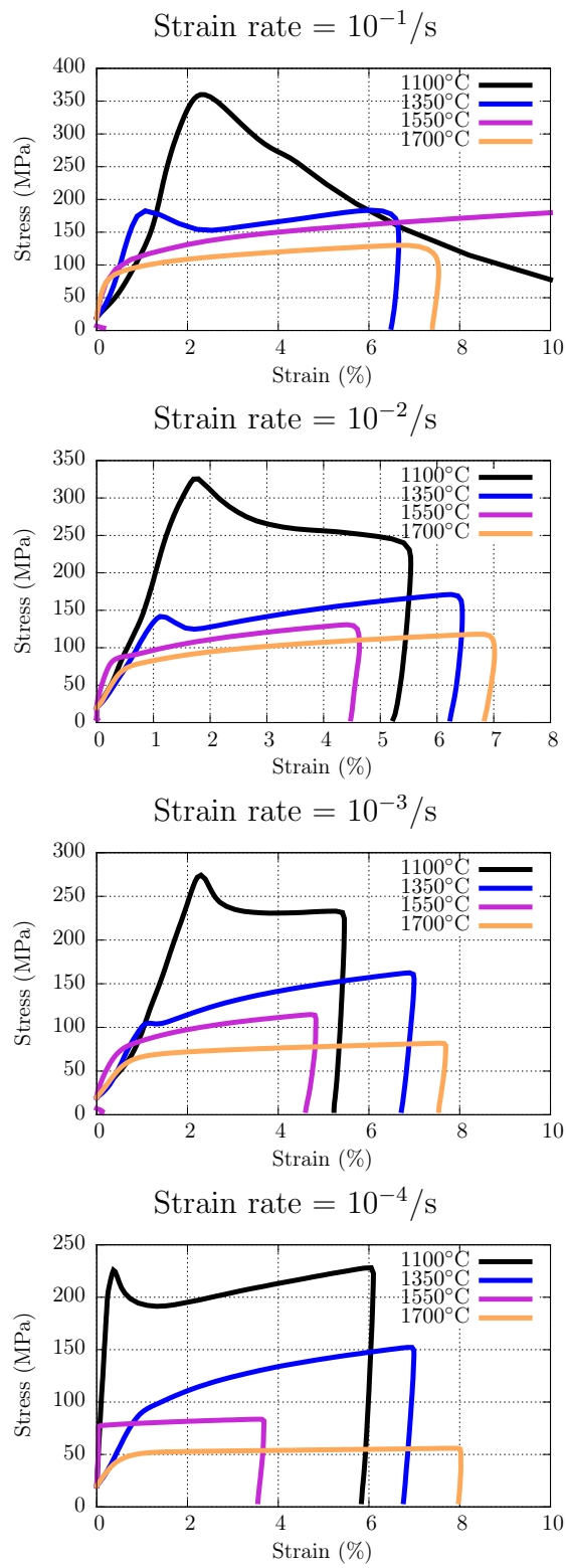
Figure 3: Stress - true strain curves obtained at different strain rates.
