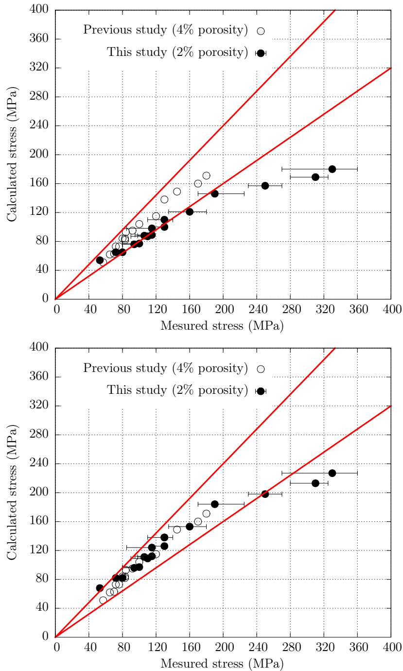
Figure 11: Calculated and measured compression stresses for two \text{UO}_2 with porosities 2% (this study) and 4% [26]. Top graph: \sigma_0 = 5 MPa for both materials. Bottom graph: \sigma_0 = 6.3 MPa for the 2% porosity \text{UO}_2 , \sigma_0 = 5 MPa for the 4% porosity \text{UO}_2 . The solid lines indicate the \pm 10\% confidence interval. The horizontal bars give the stress peak magnitude.
