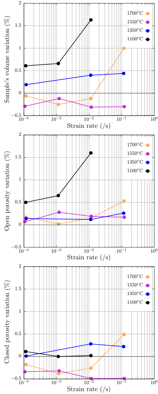
Figure 7: Evolution with temperature and strain rate of the samples' volume (top), open porosity (center), and closed porosity (bottom).
