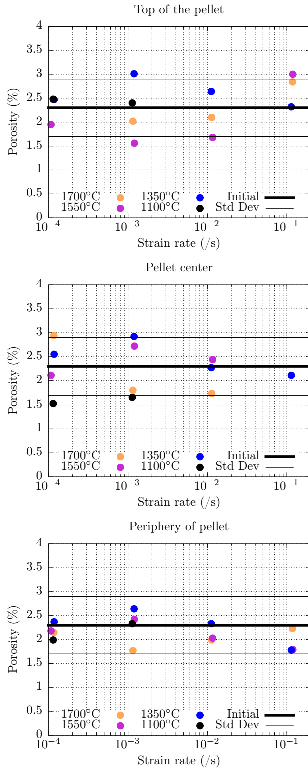
Figure 8: Post-test surface porosities at the top, periphery and center of the samples.
