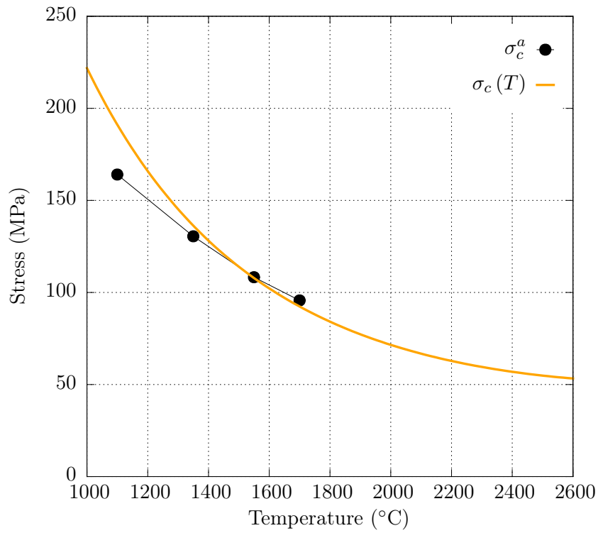
Figure 13: Evolution of the GB yield stress in compression in function of temperature. The maximum equivalent stresses \sigma_c^a = \frac{1+\tau}{2\tau}(\sigma_{eq} + \omega\sigma_m) calculated in the FE simulations during the tests performed at 10^{-1}/s are also indicated.
