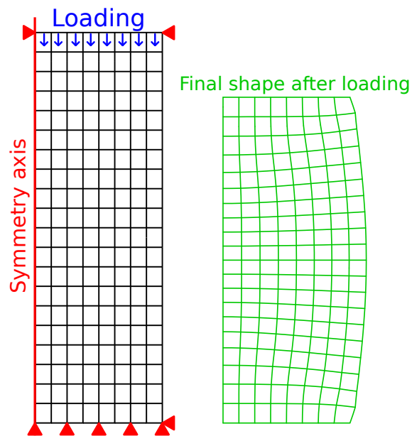
Figure 14: Mesh and boundary conditions in the simulations of the strain-driven compressive test.
