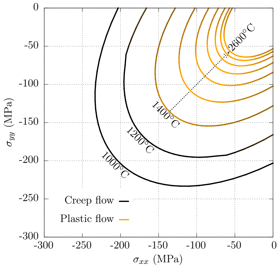
Figure 20: Biaxial yield surface obtained at an equivalent strain rate of 10/s showing the temperature and stress domains where plasticity (bright lines) or viscoplasticity (dark lines) control the material behaviour.
