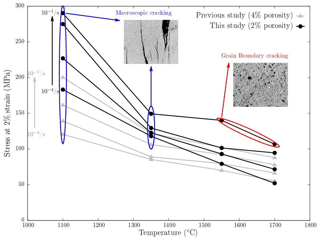
Figure 10: Synthesis of the test results in terms of stress at 2% strain versus temperature for all the strain rates, including data from a previous study on a UO_2 with a 4% initial porosity [26].
