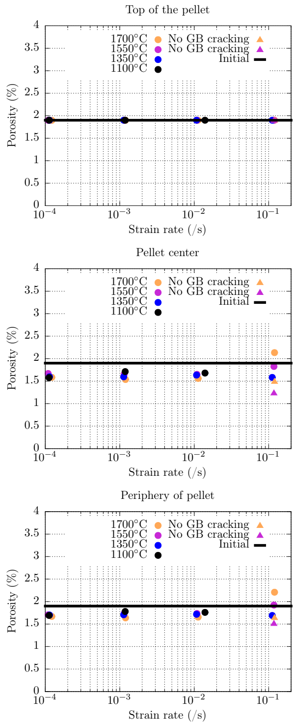
Figure 17: Calculated porosities at the top, center and periphery of the samples after all the tests.
