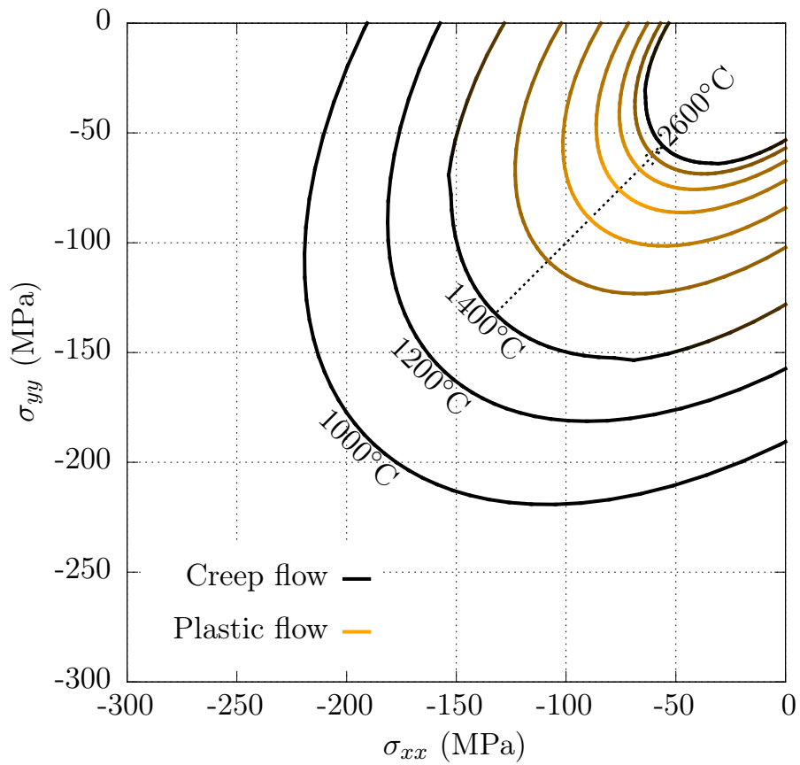
Figure 19: Biaxial yield surface obtained at an equivalent strain rate of 1/s showing the temperature and stress domains where plasticity (bright lines) or viscoplasticity (dark lines) control the material behaviour.
