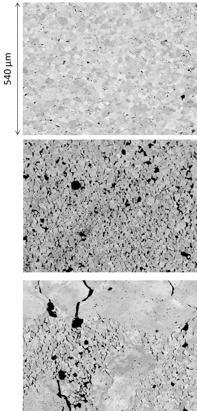
Figure 9: SEM images of the pellet center after testing at 10^{-1}/s and 1350^{\circ}C (top), 1550^{\circ}C (middle) and 1700^{\circ}C (bottom)
