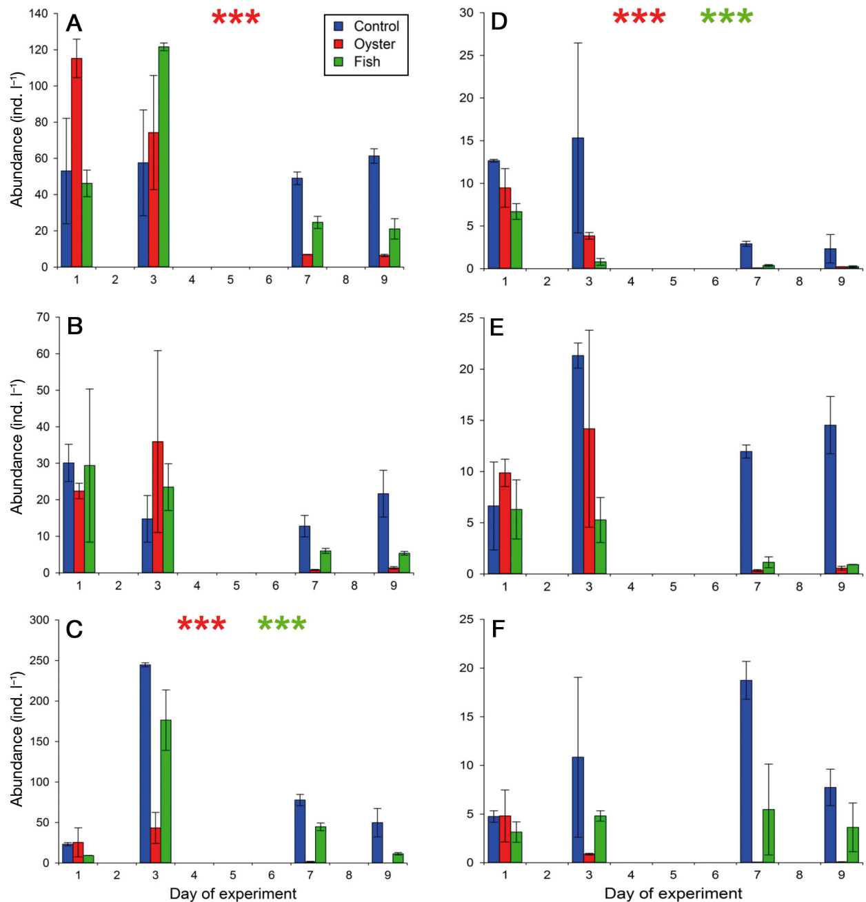
Fig. 5. Abundance (means, with error bars showing range, n = 2) of the 6 most abundant metazooplankton groups and species (ind. l -1 ) during the experiment in the Oyster, Fish, and Control mesocosms: (A) cyclopoid nauplii, (B) calanoid nauplii, (C) lamellibranch larvae, (D) gastropod larvae, (E) Oithona nana , and (F) Synchaeta triophthalma . Red and green asterisks: significant difference (p < 0.05) between the Oyster or Fish mesocosms, respectively, and the Controls for the whole experiment
