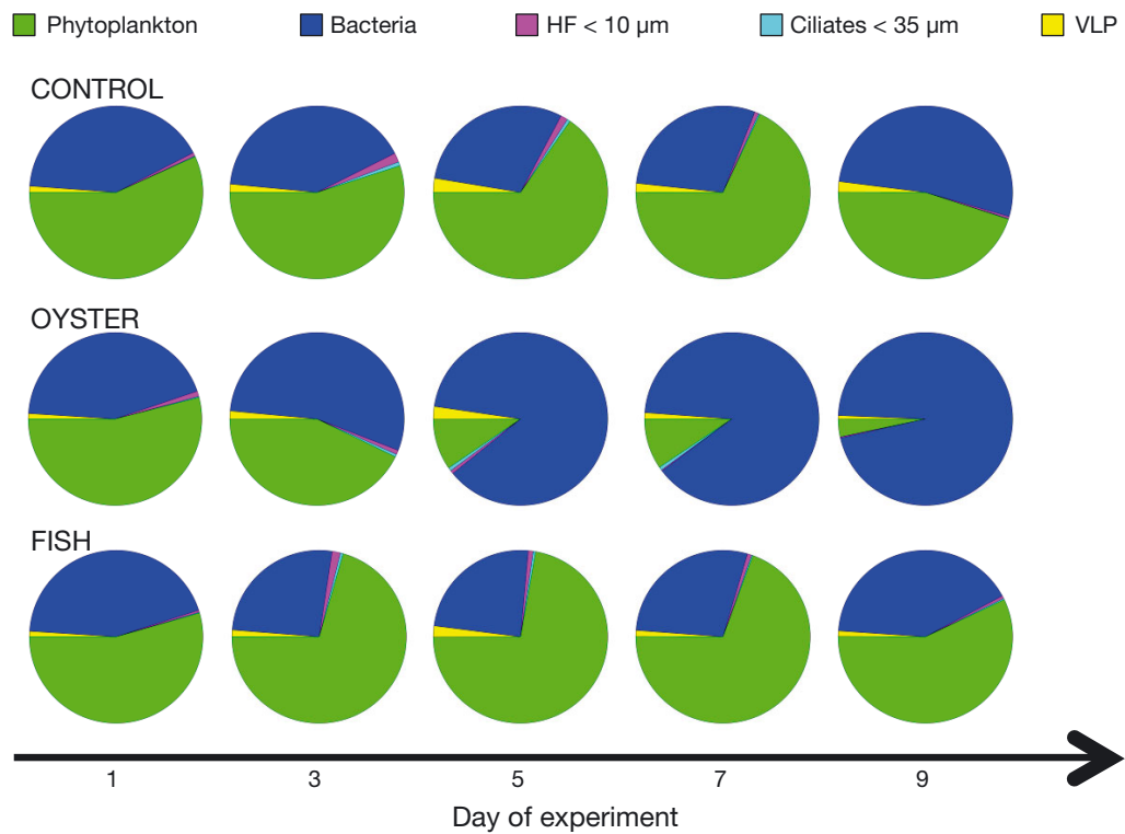
Fig. 7. Mean (n = 2) of carbon partitioning of the microbial food web components in the Control, Oyster, and Fish mesocosms on Days 1, 3, 5, 7, and 9 of the experiment. Partitioning of phytoplankton is shown in green, heterotrophic bacteria in dark blue, heterotrophic flagellates <10 µm (HF) in pink, ciliates <35 µm in light blue, and virus-like particles (VLP) in yellow
