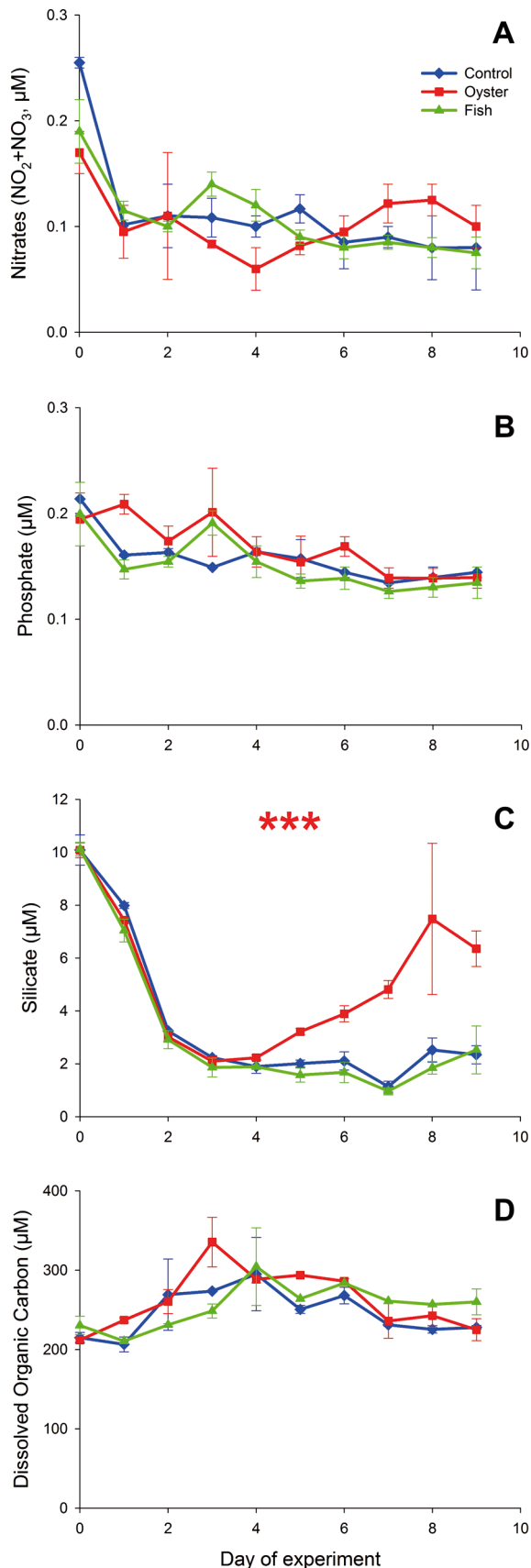
Fig. 2. Concentrations (means, with error bars showing range, n = 2) of (A) nitrates (nitrite and nitrate: NO 2 - +NO 3 - ), (B) phosphate (PO 4 3- ), (C) silicate (SiO 4 4- ), and (D) dissolved organic carbon (DOC) for the Oyster, Fish, and Control mesocosms in the course of the experiment. Red asterisks: significant difference (p ≤ 0.05) between the Oyster and Control mesocosms for the whole experiment
