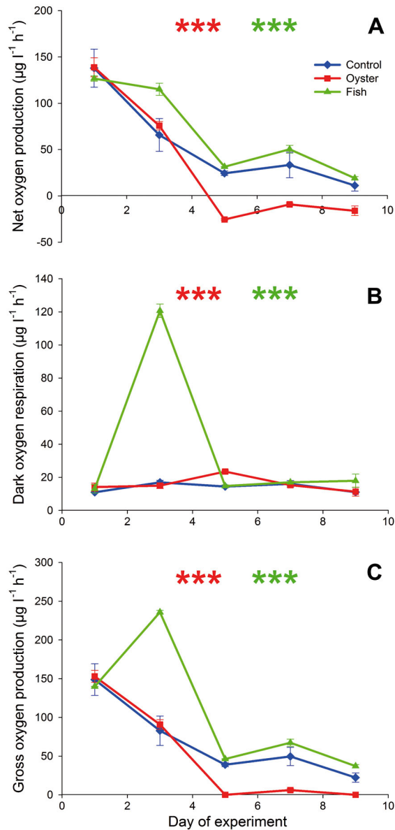
Fig. 3. Concentrations of (A) net oxygen community production (means, with error bars showing range, n = 2 ), (B) dark oxygen respiration of the microbial community measurement, and (C) gross oxygen production (means, with error bars showing range, n = 2 ) calculated from light/dark incubations, in the Oyster, Fish, and Control mesocosms during the experiment. Red and green asterisks: significant difference ( p \leq 0.05 ) between the Oyster or Fish mesocosms, respectively, and the Controls for the whole experiment
