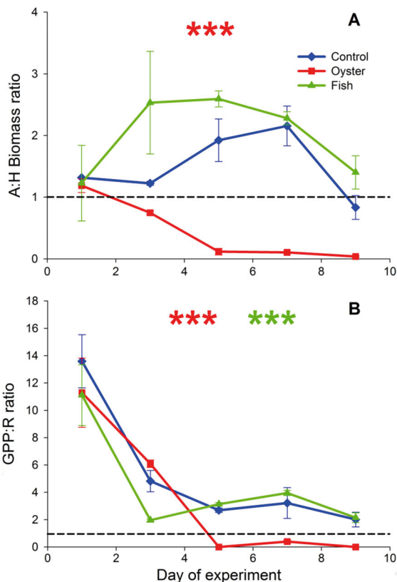
Fig. 8. Dynamics of microbial food web (A) structural index of autotroph:heterotroph (A:H) C biomass ratios and (B) functional index of gross primary production:respiration (GPP:R) ratios in the Oyster, Fish, and Control mesocosms during the experiment. Data are the means with error bars showing range ( n = 2 ). The black dashed lines represent a ratio of 1. Red and green asterisks: significant difference ( p \leq 0.05 ) between the Oyster or Fish mesocosms, respectively, and the Controls for the whole experiment
