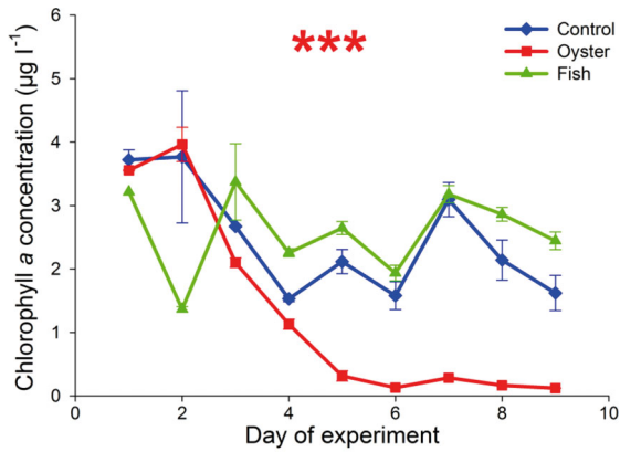
Fig. 6. Chlorophyll a concentrations (means, with error bars showing range, n = 2) measured by HPLC in the Oyster, Fish, and Control mesocosms during the experiment. Red asterisks: significant difference ( p \leq 0.05 ) between the Oyster and Control mesocosms for the whole experiment
