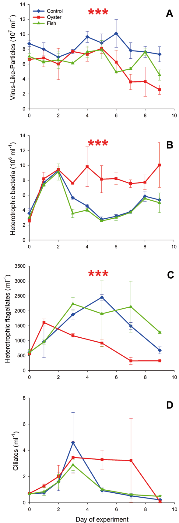
Fig. 4. Abundances (means, with error bars showing range, n = 2 ) of (A) virus-like particles, (B) heterotrophic bacteria, (C) heterotrophic flagellates <10 \mu\text{m} , and (D) ciliates <35 \mu\text{m} in the Oyster, Fish, and Control mesocosms during the experiment. Red asterisks: significant difference ( p \leq 0.05 ) between the Oyster and Control mesocosms for the whole experiment
