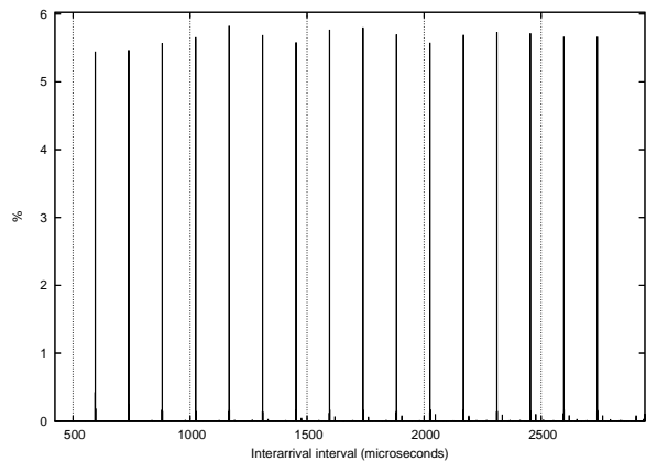
Figure 12: Linksys WRT 54GL, default configuration.
