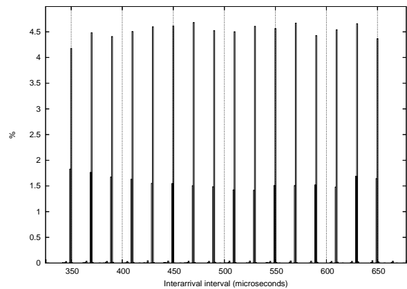
Figure 23: Linksys-Broadcom card.
