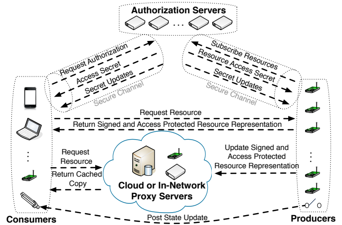
Fig. 1. OSCAR, a producer-consumer security model for IoT based on object security.
