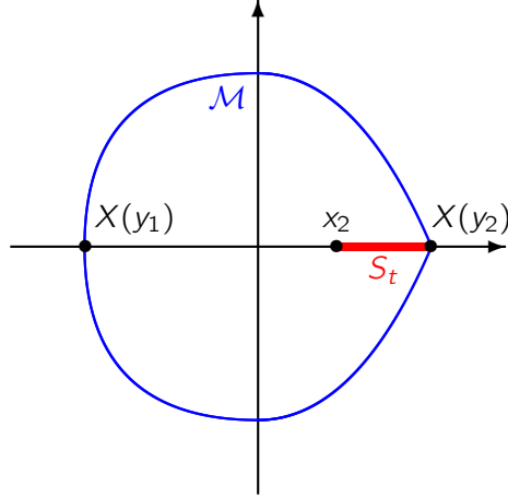
Figure 2. The curve \mathcal{M} = X([y_1, y_2]) is symmetrical w.r.t. the real axis. It is smooth everywhere except at X(y_2) , where it may have a corner point (if and only if t = t_0 ). Any 1/p , with p point of the red segment S_t , is the exponential growth of a harmonic function
