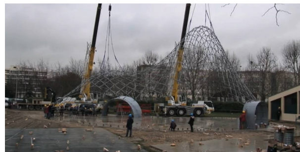
Figure 2: Cathedrale Ephemere de Creteil. Primary grid deformed elastically and about to be attached to boundary conditions.
