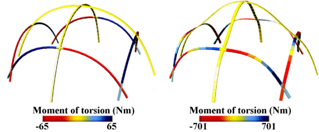
Figure 13: Equilibrium shapes of two gridshells identical at the flat stage. On the left, the beams have square-sections, on the right the sections are oblong. The shapes are rather different and the moments of torsion really different.
