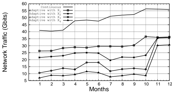
Fig. 4. Network Bandwidth Consumption
