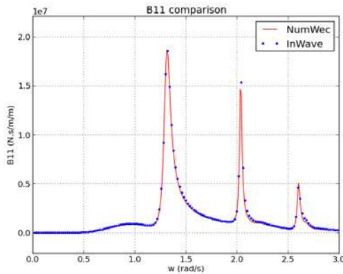
Figure 5: F-3OF Radiation damping (1,1)
