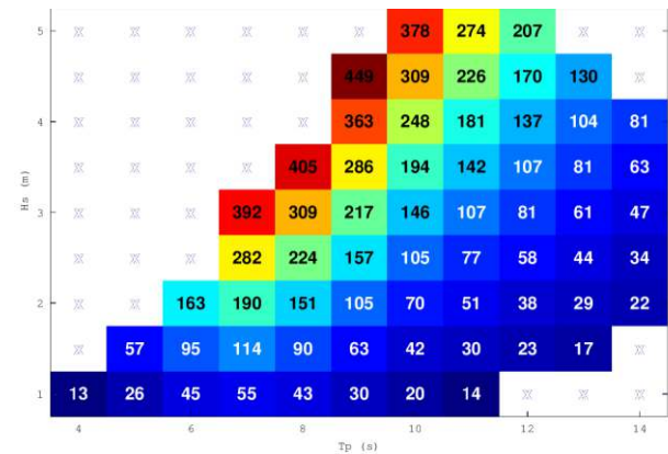
Figure 10: F-3OF power matrix obtained with InWave
