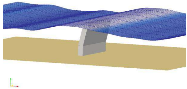
Figure 19: B-OF device in irregular waves on InWave
