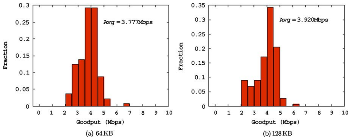
Fig. 2. Moving scenario (vehicles move on a straight road): goodput results.
