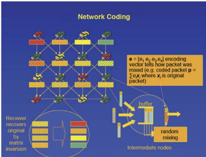
Fig. 3. Random Linear Network Coding in CodeTorrent. (For interpretation of the references to color in this figure, the reader is referred to the web version of this article.)
