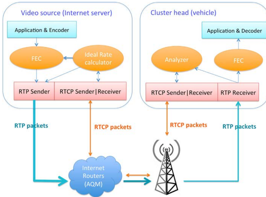
Fig. 10. System architecture of segment 1: unicast from source to cluster head.
