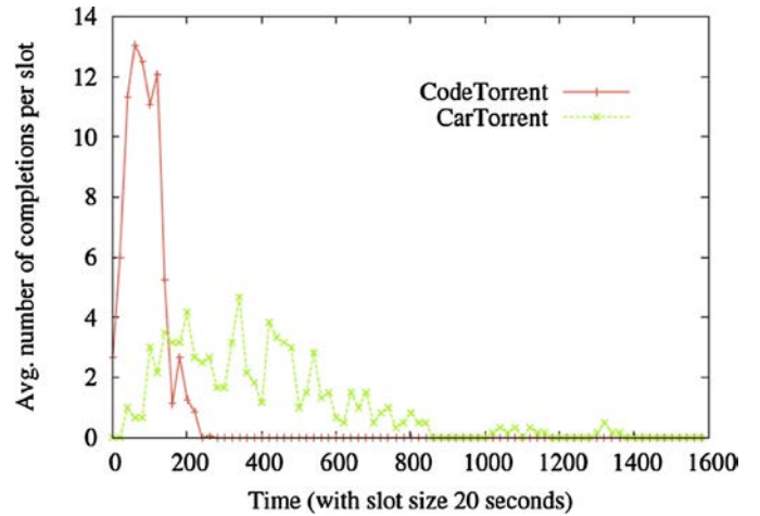
Fig. 4. Comparison of downloading time between CarTorrent and CodeTorrent.
