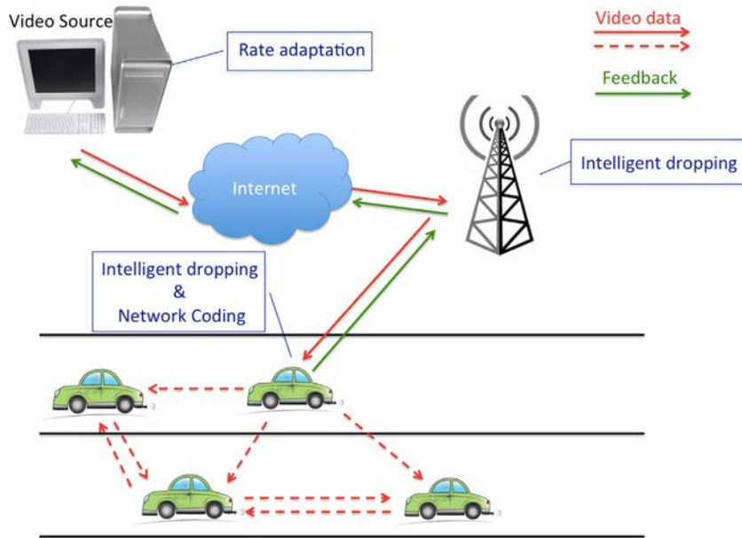
Fig. 9. System architecture for VANET video congestion control.
