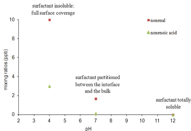
Figure 4. Evolution of gaseous nonenal and nonenoic acid concentration as a function of the pH of the solution.
