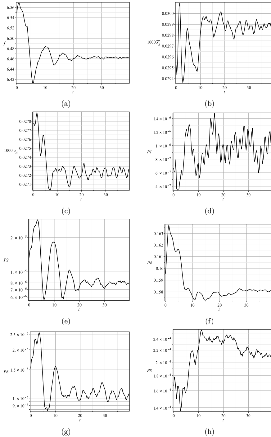
Figure 33: Details of the thread of Fig. 32: beam frequency (BF) (a), point A's mean position (b), point A's amplitude (c), and point A's spectral components at: 1 \times \text{BF} (d), 2 \times \text{BF} (e), 4 \times \text{BF} (f), 6 \times \text{BF} (g), 8 \times \text{BF} (h).
