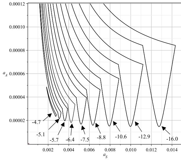
Figure 16: Stationary condition, a_A (point A's amplitude) against a_S (stationary motion's amplitude). A few curves solution for the smoothed model, for various values of F_0 , denoted by arrows in the graph. Parameter values are the same as in Fig. 14.
