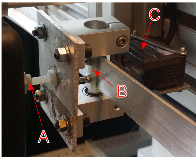
Figure 23: Shaker. A: nylon rod and nuts, B: axis of the revolute joint, C: control beam's position sensor.
