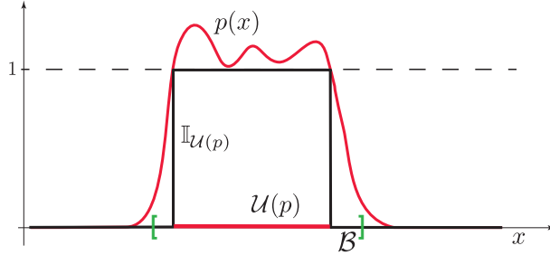
Figure 1: Illustration of Chebychev's inequality: the polynomial is always greater or equal than the indicator function of p(x) \geq 1 , hence the integral of p over \mathcal{B} is always an upper bound of the volume of \mathcal{U}(p) .
