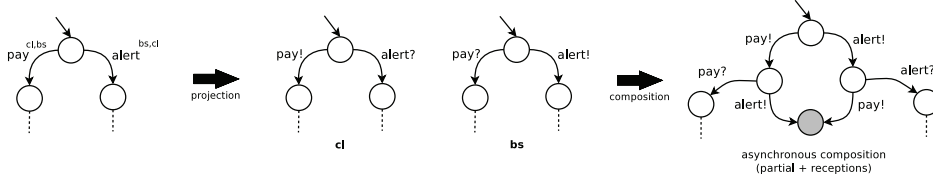
Fig. 12. Example of a Non-Repairable Choreography
