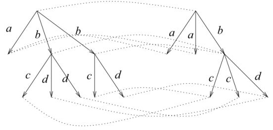
Figure 1: Two bisimilar graphs (taken from [5]).
