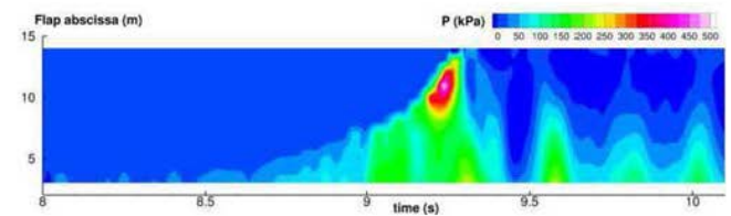
Fig. 16 Evolution of the measured pressure on the flap in the time-space plane for the case BT80.
