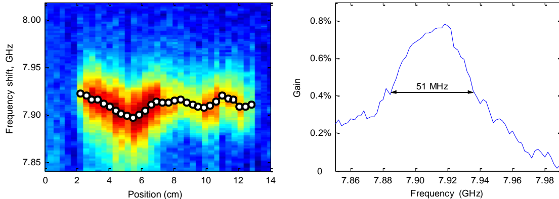
Figure. 2. Experimental results: (a) Distributed Brillouin gain spectrum measured along the 13 cm-long chalcogenide microwire (white markers show the peak of the Brillouin resonance). (b) Local Brillouin gain spectrum in the middle of the microwire.
