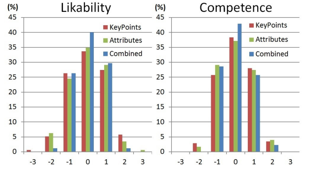
Fig. 4. Classification errors ( CCE ) for likability and competence, using different feature sets: facial keypoints (red), high level attributes (green) and global feature set (attributes and keypoints, blue).
