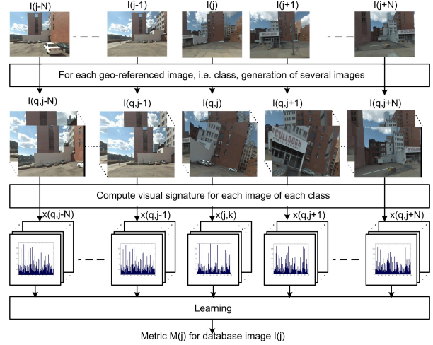
Figure 5. Creation of simulated similar and dissimilar examples in order to learn for each geo-referenced image database I_j a metric M_j .
