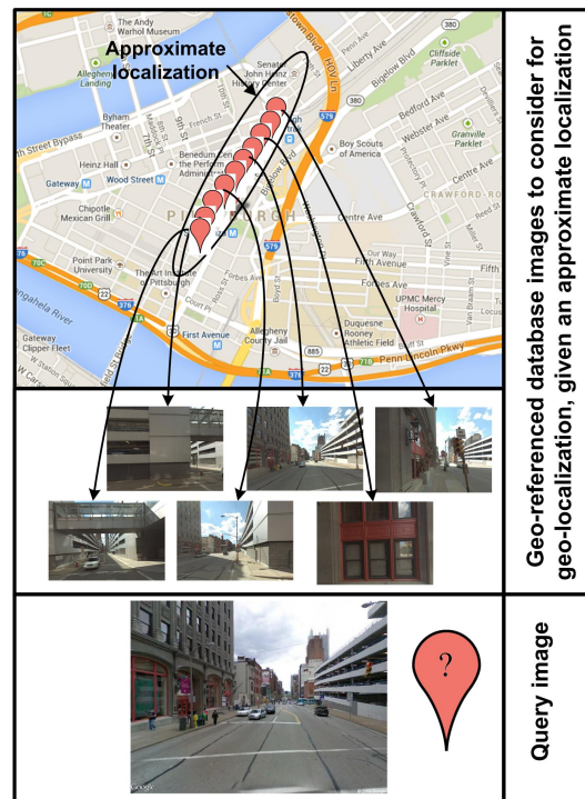
Figure 1. Our system aims at answering the following question: knowing a roughly position of the vehicle in a street and the scene being observed by the vehicle's camera, can we determine where it is exactly along the street?
