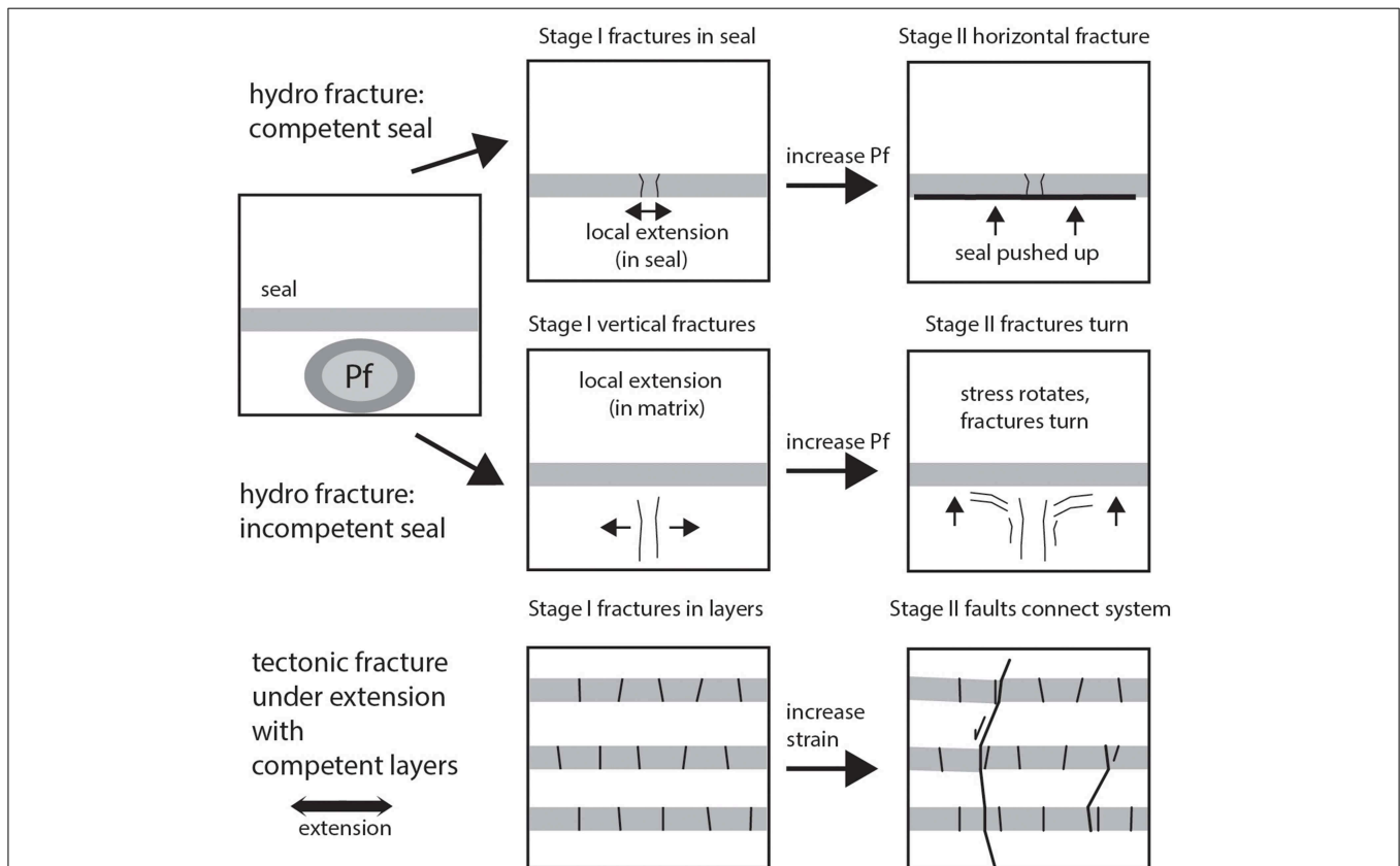
FIGURE 9 | Summary figure illustrating different fracture patterns that develop below and in a competent vs. an incompetent seal and fracture and fault patterns that develop in a layered sequence that is extended. Hydrofractures tend to develop around sources of high fluid pressures where fluid pressure gradients fracture the matrix or bend competent layers leading to fractures. During extension fractures are well spaced along the beds and at higher strain faults connect different layers and drain systems of high fluid pressure.
