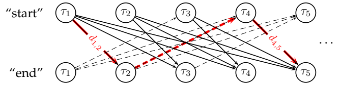
Figure 11. Graph construction for the maximum-weight path formulation of the sampling problem (one operator, with silence periods). Solid edges have weights equal to the corresponding distance proofs ( d_{i,j} is the short for d(A_i, A_j) ). Dashed edges have zero weights. The thick, red path shows an example of a set of sampling points: The user starts a distance proof at time \tau_1 (by collecting location proofs), which she ends at time \tau_2 thus collecting a proof of value d_{1,2} ; she then starts a new distance proof at time \tau_4 (thus observing a silence period) which she ends at time \tau_5 . The total weight of this path is d_{1,2} + d_{4,5} .
