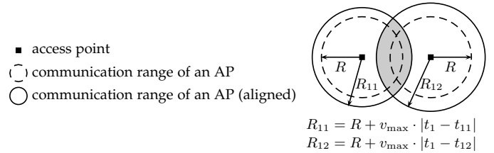
Figure 2. Time alignment of location proofs LP_{11} and LP_{12} at time t_1 . At t_1 , the user was in the gray area defined by the intersection of the two solid discs.
