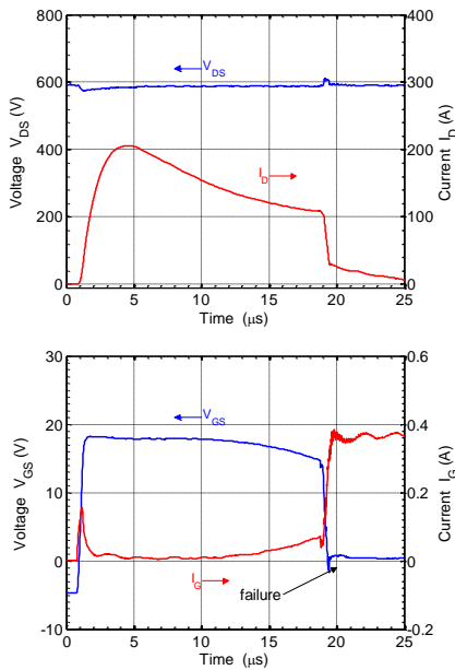
Fig. 5 Destructive test of C-MOSFET#1, R_G = 47 \Omega , T_{CASE} = 25^\circ C .
