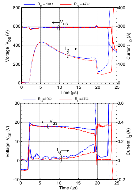
Fig. 8 Failure of C-MOSFET: drain and gate waveforms, at T_{CASE} = 25^\circ\text{C} for R_G = 10 \Omega and 47 \Omega .
