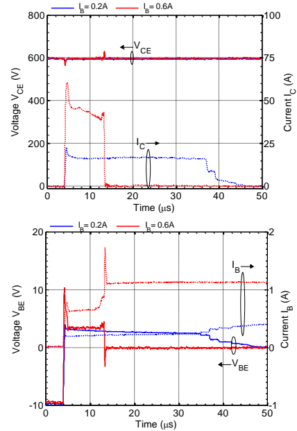
Fig. 3 Failure of BJT for T_{CASE} = 25^\circ\text{C} .
