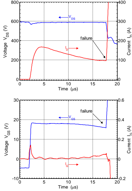
Fig. 4. Destructive test for A-MOSFET, R_G = 47 \Omega , T_{CASE} = 25^\circ C .
