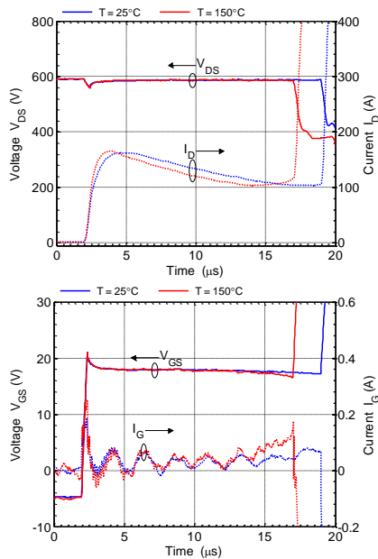
Fig. 6 Failure of A-MOSFET: drain and gate waveforms, for R_G = 10 \Omega , T_{CASE} = 25^\circ\text{C} and 150^\circ\text{C} .
