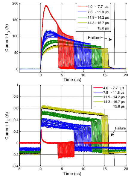
Fig. 10 Ageing of SiC B-MOSFETs during repetitive SC by increasing SC duration with a low time step.
