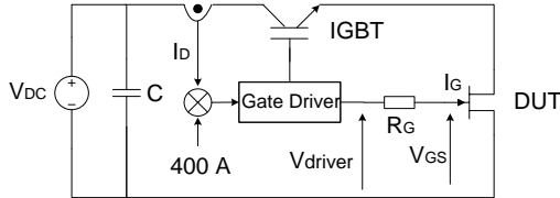
Fig. 1 Schematic of short-circuit test circuit for MOSFET
