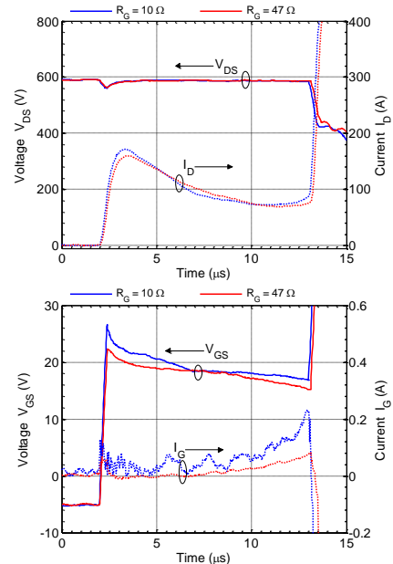
Fig. 7 Failure of B-MOSFET: drain and gate waveforms, at T_{CASE} = 150^\circ\text{C} for R_G = 10 \Omega and 47 \Omega .
