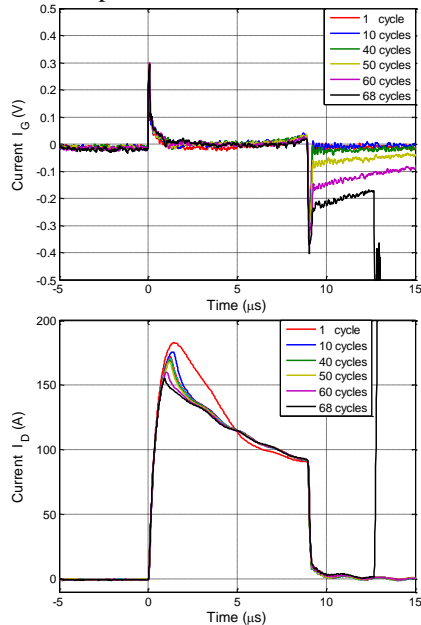
Fig. 11 Ageing of B-MOSFETs during repetitive SC, t_{SC} = 9\mu\text{s} repetition, R_G = 10\ \Omega , T_{CASE} = 25^\circ\text{C}
