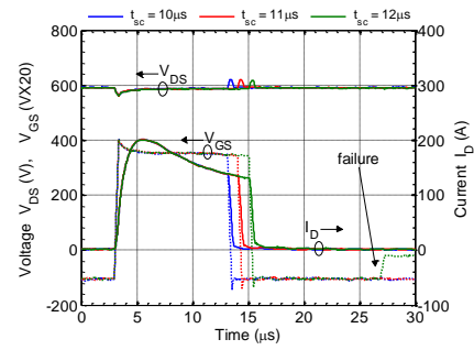
Fig. 9 Short circuit behavior of C-MOSFET for R_G = 10 \Omega and T_{CASE} = 150^\circ\text{C} .
