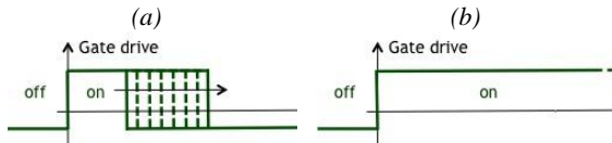
Fig. 2 Robustness tests under (a) short-circuit and (b) current limitation.
