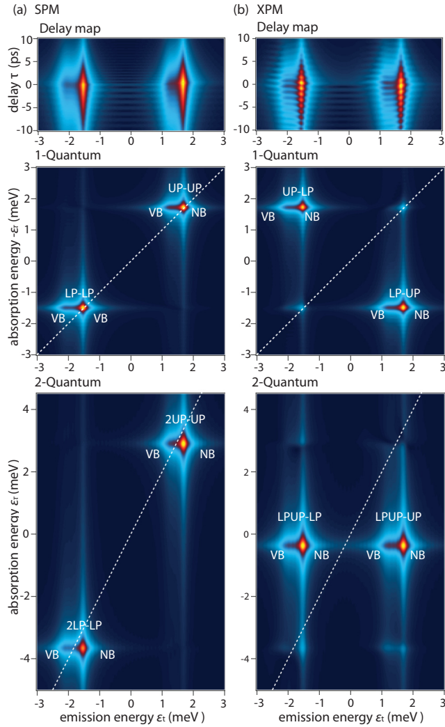
FIG. 7. (Color online) Simulated delay map |S(\tau, \epsilon_t)| and 2D FT spectrum |S(\epsilon_t, \epsilon_r)| for one-quantum and two-quantum regimes. Simulations are performed including only self-interaction (or self-phase modulation: SPM) g_X = 0 (a) and for only cross interaction (or cross-phase modulation: XPM) g_{L(U)} = 0 (b).
