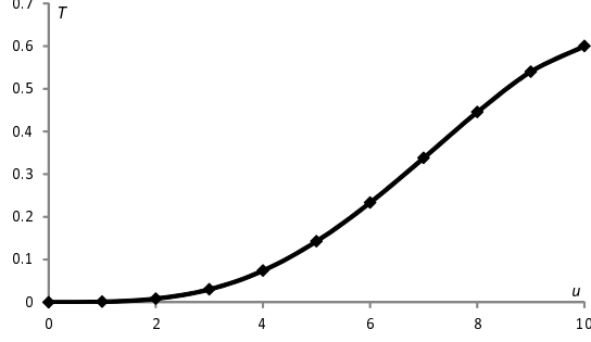
Figure 1: Email throughput ( s = 10 , \mu_0 = \mu = 0.2 , \lambda = 1.4 )
