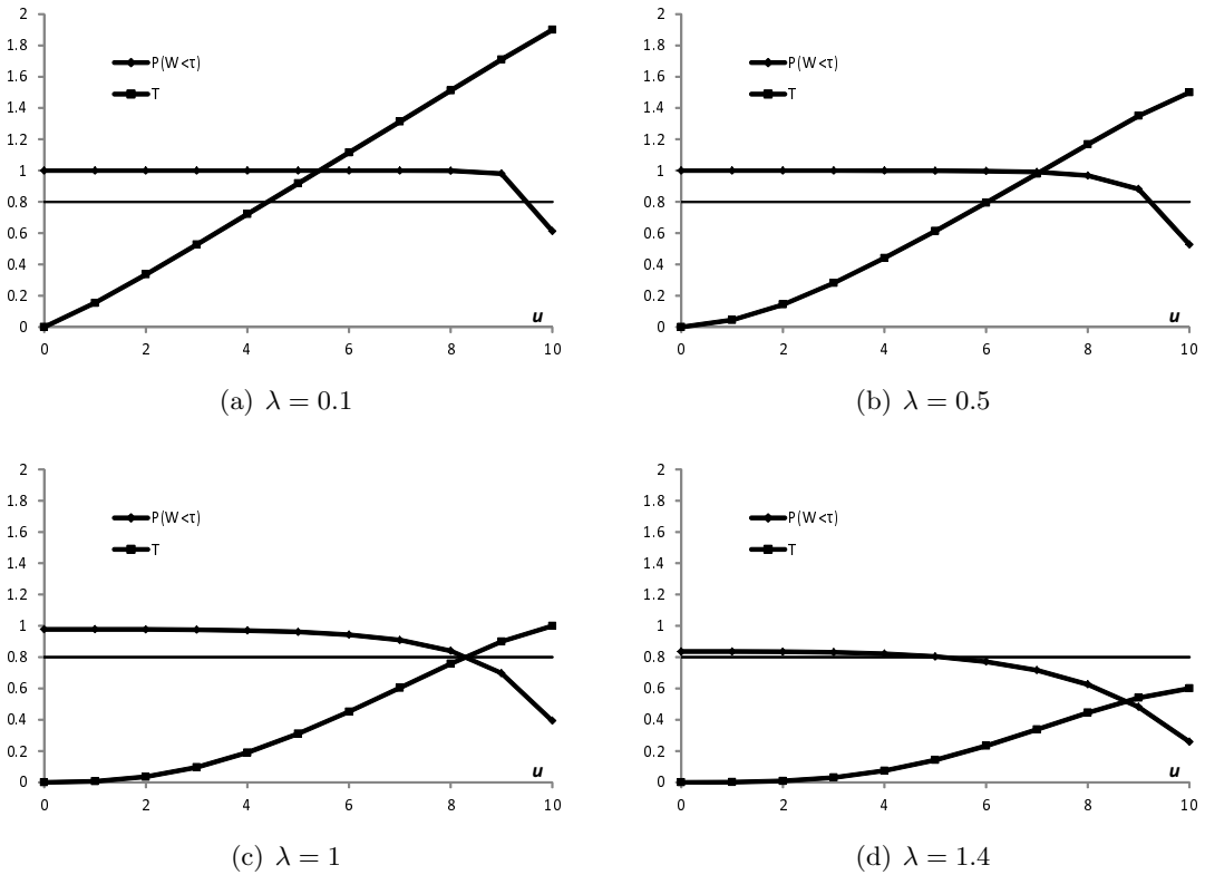
Figure 3: Performance measures ( s = 10 , \mu = \mu_0 = 0.2 , \tau = 0.5 , \alpha = 80\% )
