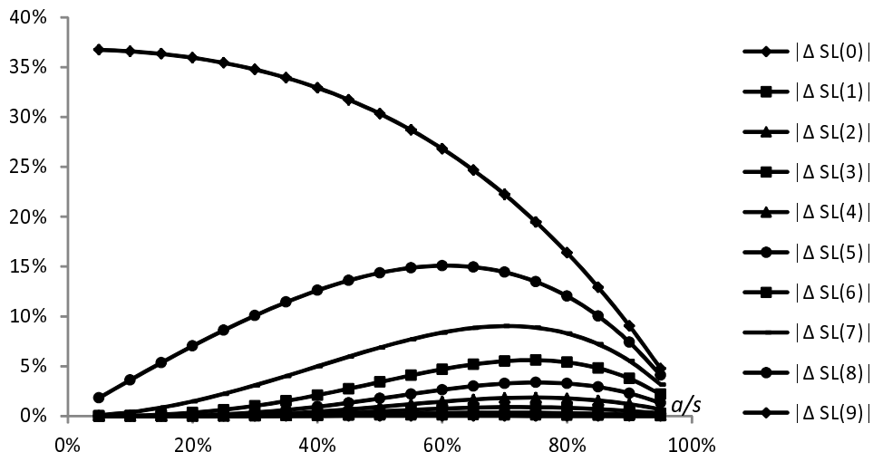
Figure 2: Sensitivity of the service Level ( s = 10 , \tau = 30 seconds, \mu = \mu_0 = 0.2 )
