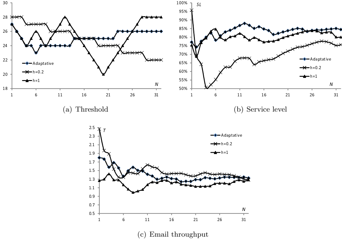
Figure 4: Evolution of the threshold, the service level and the throughput (Scenario 2)
