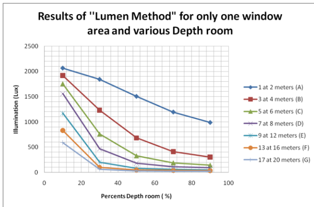
Fig. 4: Results of ‘‘Lumen Method’’ for only one window are and various depth room
