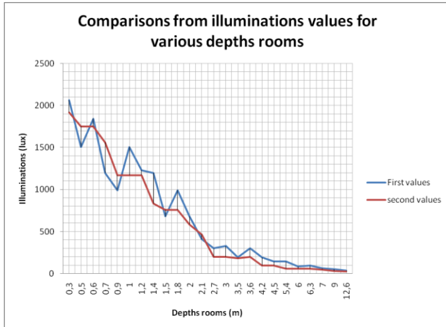
Fig. 6: Comparison from illuminations values for various depths rooms
