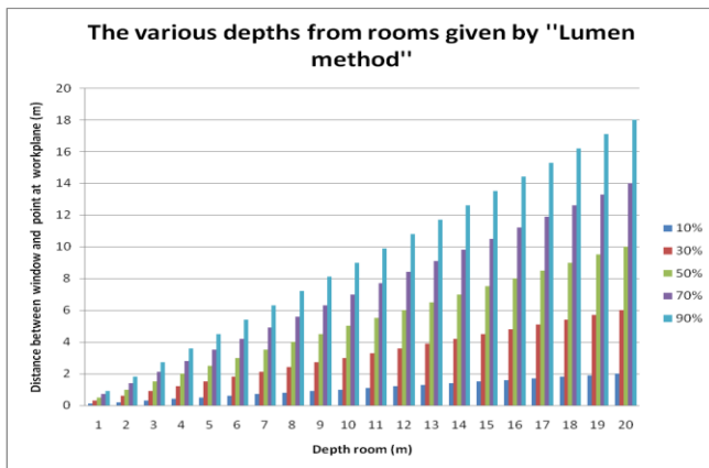
Fig. 5: The various depths from rooms given by ‘‘Lumen method’’
