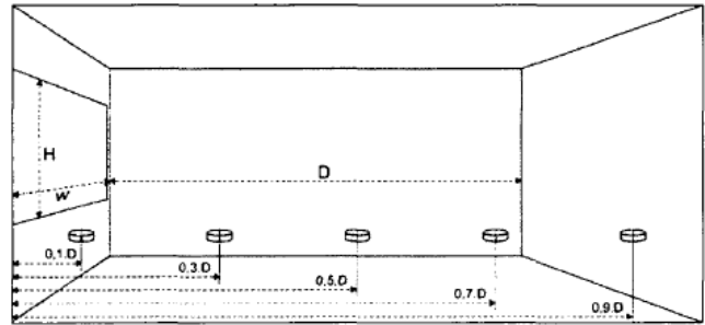
Fig. 1: Standard configuration in a room for calculating sidelighting (Lumen method) [7]
