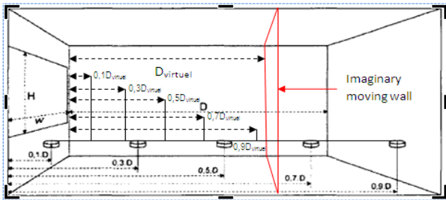
Fig. 2: proceeding for calculating sidelighting with improving "Lumen method"
