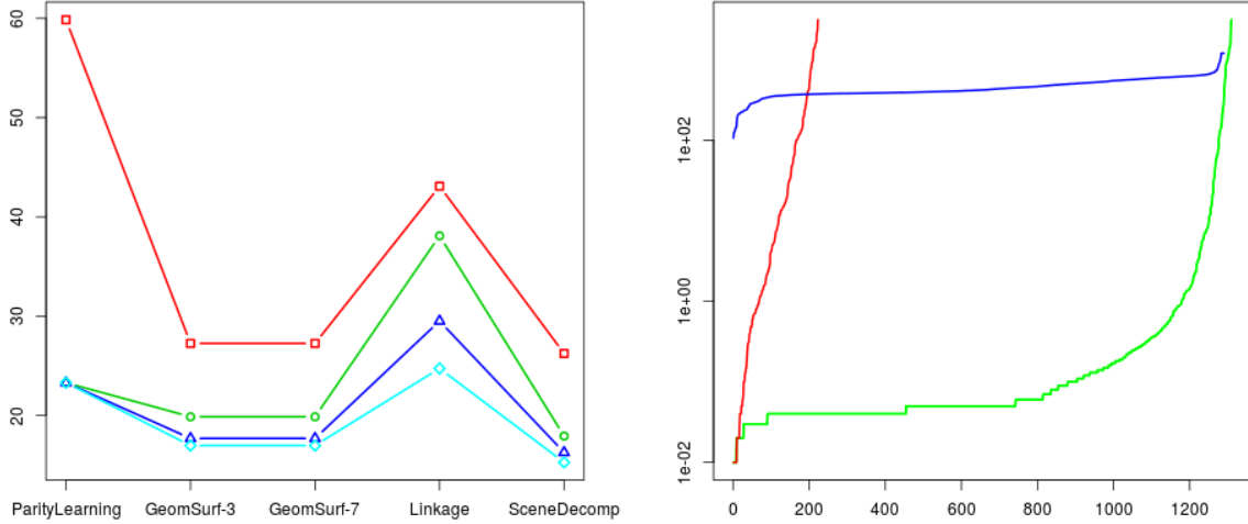
Figure 6: Left: Comparison of treewidth bounds provided by MCS (red), minimum degree (green), minimum fill-in (blue) and randomized iterative minimum fill-in (cyan) for the 5 categories of problems Right: Mode evaluation by three exact methods exploiting minimum fill-in ordering or its randomized iterative version. Number of instances solved ( x -axis) within a given CPU time (log10 scale y -axis) of ELIM (red), BTD (green), and AND/OR SEARCH (blue).
