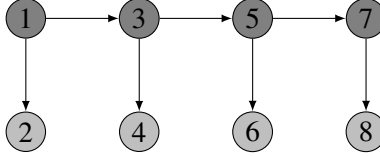
Figure 2: Graphical representation of a HMM. Hidden variables correspond to vertices 1, 3, 5, 7, and observed variables to vertices 2, 4, 6, 8.
