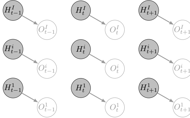
Figure 10: Graphical representation for the independent mean-field approximation of p(h, o) in a coupled HMM. Observed variables are indicated in light gray since they are not part of the variational distribution which is a distribution only on the hidden variables.
