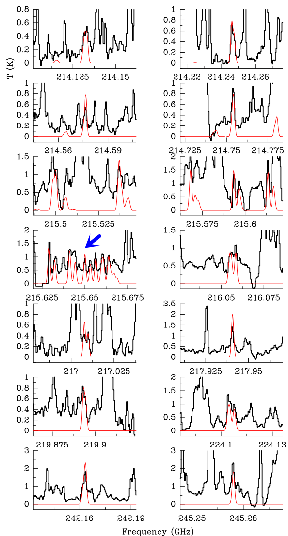
Fig. 1. Selected lines of trans Ethyl Methyl Ether, t\text{-CH}_3\text{CH}_2\text{OCH}_3 , towards Orion KL detected with the ALMA interferometer in Position A (see text). A v_{LSR} of +7.5 \text{ km s}^{-1} is assumed.
