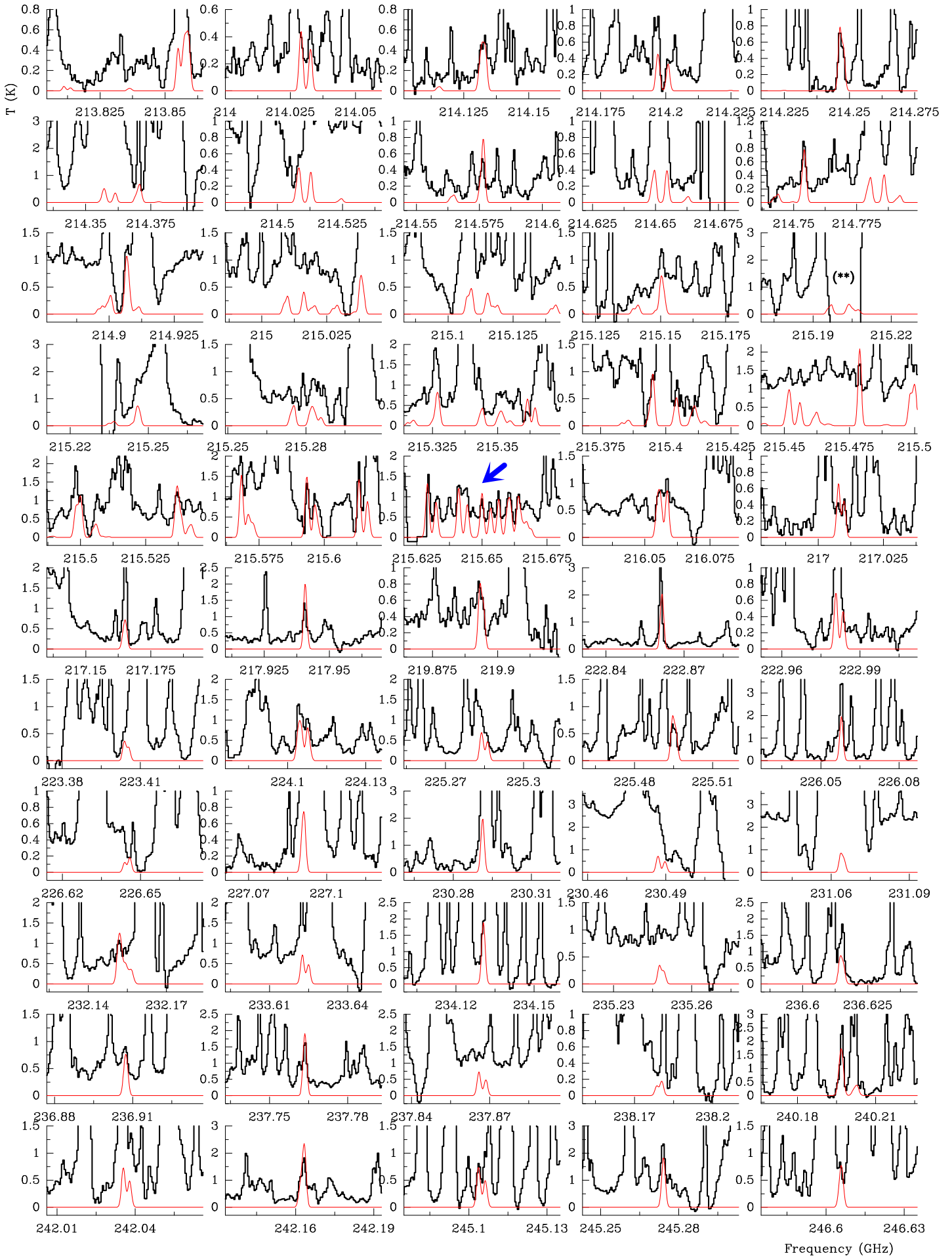
Fig. A.1. Lines of trans Ethyl Methyl Ether, t - \text{CH}_3\text{CH}_2\text{OCH}_3 , towards Orion KL detected with the ALMA interferometer in Position A (see text). (**): Features blended with SO (see Table A.1; artifacts in the spectrum due to the cleaning process). A v_{LSR} of +7.5 \text{ km s}^{-1} is assumed.
