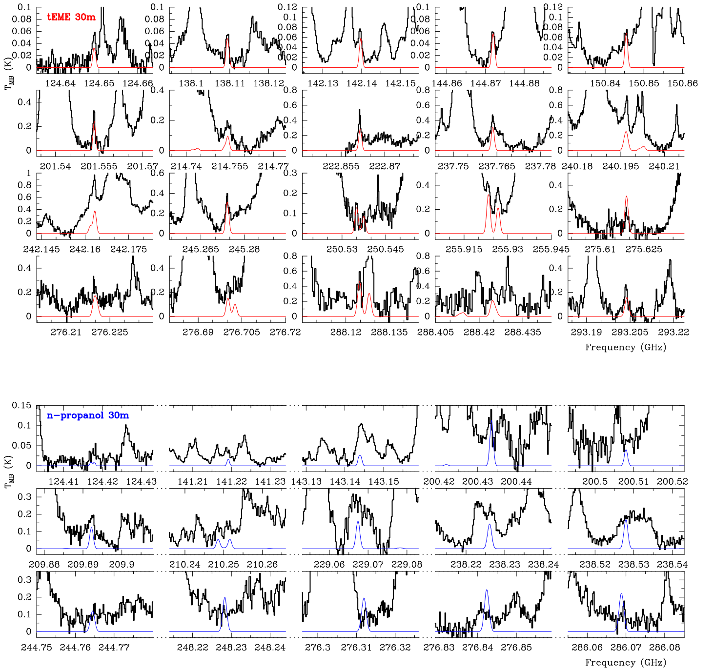
Fig. A.2. Top panel: selected lines of trans Ethyl Methyl Ether, t - \text{CH}_3\text{CH}_2\text{OCH}_3 , towards Orion KL detected with the IRAM 30m telescope. Data in the frequency range 124–151 GHz are those of the survey position. From 201 to 293.5 GHz the data are those of the CR (see Sect. 2), where the emission peak of organic saturated O-rich species such as dimethyl ether ( \text{CH}_3\text{OCH}_3 ) and methyl formate ( \text{CH}_3\text{OCOH} ) is located (Favre et al. 2011; Brouillet et al. 2013). A v_{LSR} of +7.5 \text{ km s}^{-1} is assumed. Bottom panel: selected lines of gauche-trans -n-Propanol, Gt- \text{n-CH}_3\text{CH}_2\text{CH}_2\text{OH} , towards Orion KL detected with the IRAM 30m telescope. A v_{LSR} of +7.5 \text{ km s}^{-1} is assumed.
