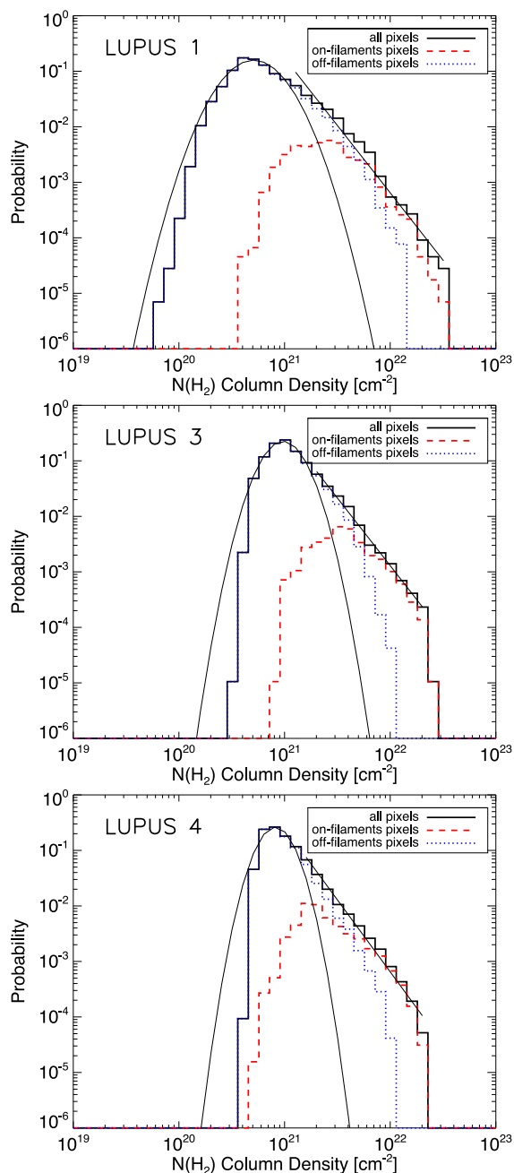
Figure 13. PDF of the Lupus 1, 3, and 4 clouds. The black histogram represents the distribution of all the pixels of the map, the red, dashed histogram the distribution of the pixels belonging to filaments excluding pixels around dense cores and the blue dotted histogram the distribution of the pixels not belonging to filaments excluding pixels around dense cores. The lognormal and power-law fit to the PDFs are also shown as continuous black lines.
