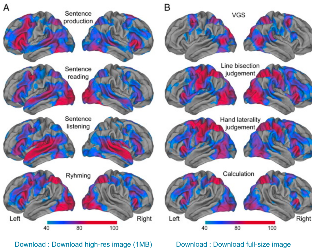
Fig. 1. Activation probability maps computed on the subsample of right-handed individuals of the BIL&GIN ( N = 140 ) for various contrasts of the language (panel A) and spatial/numerical (panel B) fMRI sessions. Each probability map is built from individual activation maps using a zero-threshold. Resulting probability maps are displayed using a 40% lower threshold, i.e., keeping only voxels showing activation in at least 40% of the sample.
