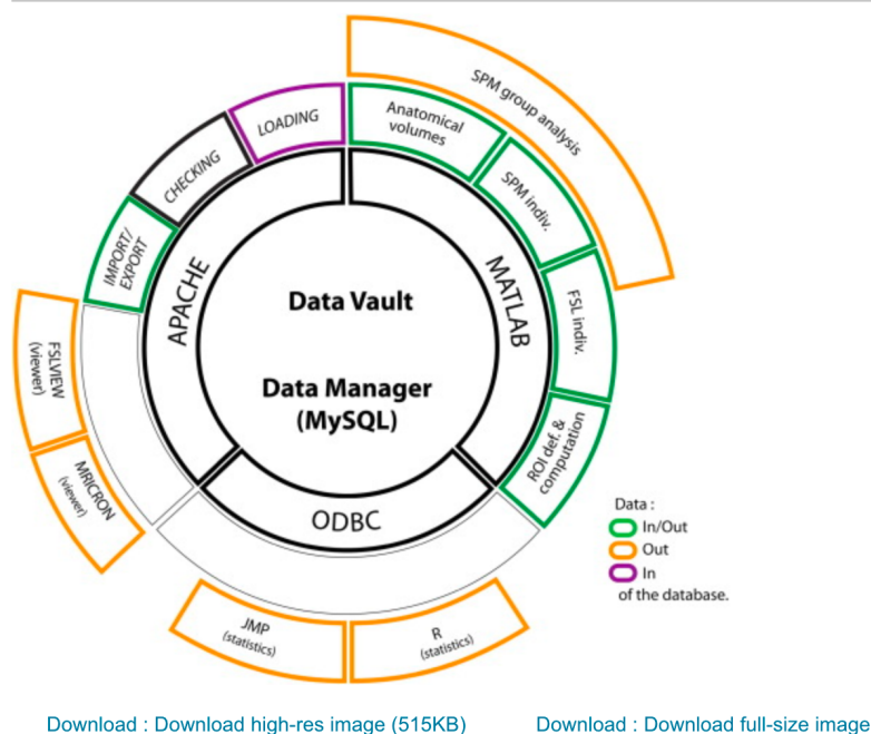
Fig. 2. GINdb, the BIL&GIN management system. Management of the database is organized in 3 layers. The core of GINdb is based on MySQL ( http://www.mysql.com ) and is linked to the software through a 1st layer made of 3 interfaces namely Matlab©, Apache ( http://apache.org ), and ODBC ( http://www.mysql.com ). A 2nd layer includes the software that accesses the database, while a 3rd layer concerns software interfaced for group-level statistical analysis (SPM, JMP©, R ( http://cran.r-project.org )) and visualization purposes (MRicron, http://www.sph.sc.edu/comd/rorden/MRicron ).
