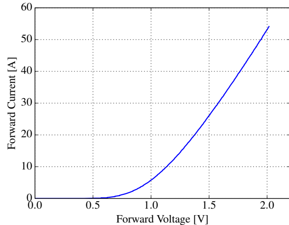
Figure 5: Forward characteristic of the embedded die
