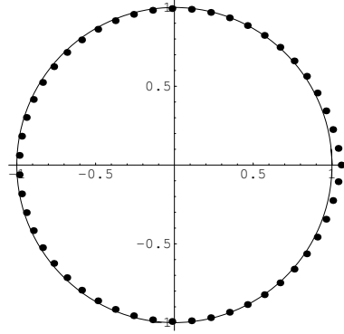
Figure 1. The roots (black bullets) of G_n^*(X) (represented here with n = 51 ) are uniformly distributed near |z| = 1 according to the theory of Erdős-Turán-Amoros-Mignotte. A slight bump appears in the half-plane \Re(z) > 1/2 in the neighbourhood of 1, at the origin of the different regimes of asymptotic expansions. The dominant root of G_n^*(X) is the Perron number \theta_n^{-1} > 1 .
