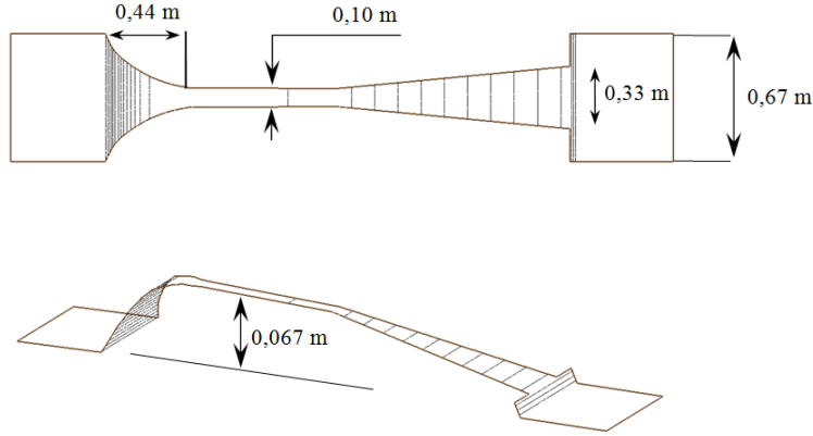
Figure 8: Test 4 - Dimensions of the Venturi flume used in the experiment. Top: plan view. Bottom: bird eye's view with a vertical scale magnified by a factor 5.
