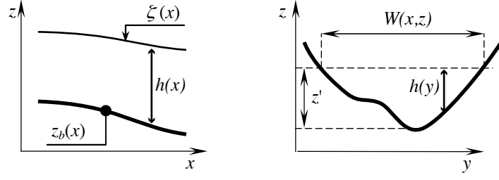
Figure 1: Channel geometry. Left) longitudinal view: bottom and water elevation. Right) transversal view: channel width and depth.
