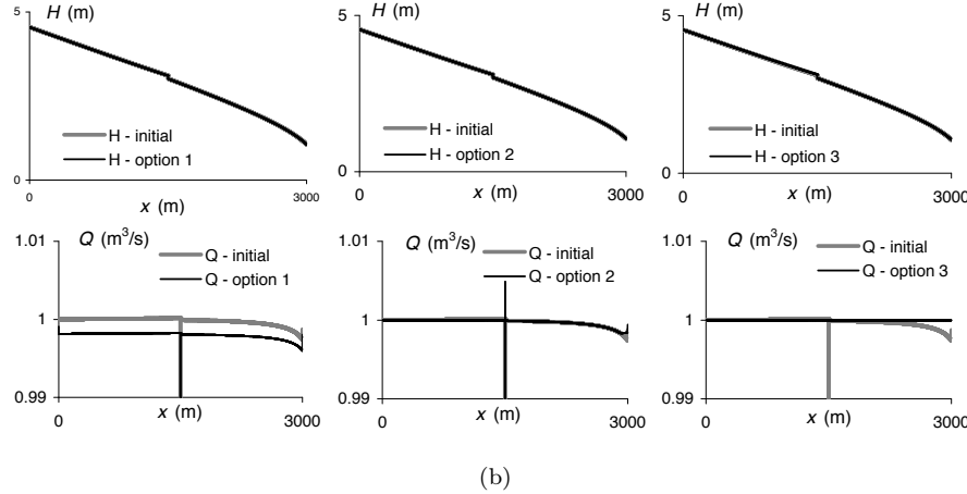
Figure 3: Test 1b - steady state flow in a prismatic, rectangular channel with an arbitrary singular head loss in the middle of the channel. Top: water elevation z and hydraulic head H , down: discharge Q obtained with \mathbf{V} = \mathbf{U} (Initial) and with the three different AVB options, using a) HLL solver, b) Roe's solver (identical to Q -scheme).
