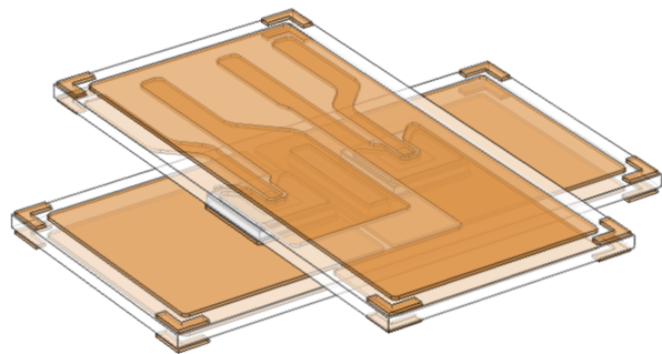
Figure 4: 3D view of the module of fig. 3 showing the internal layout and the two SiC JFET dies.
