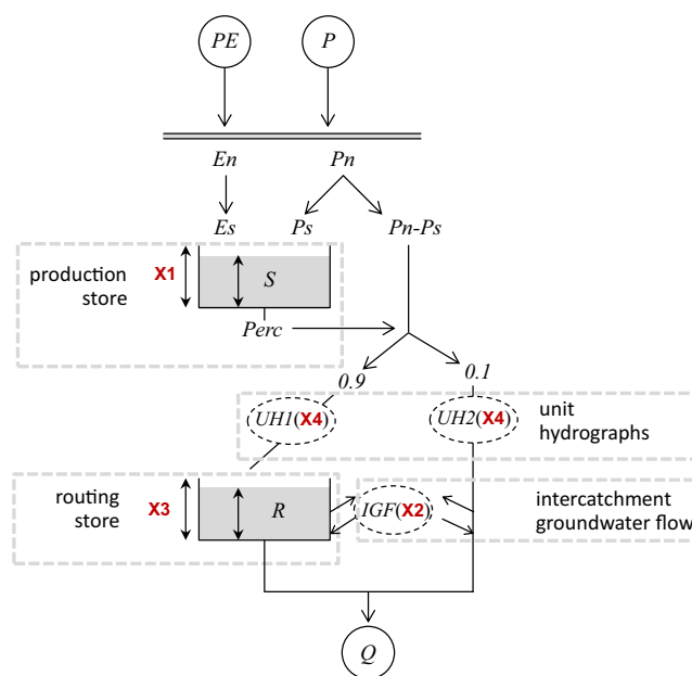
Figure 1. Schematic diagram of the structure of the four-parameter GR4J model (X1–X4 are model parameters; PE: potential evapotranspiration, P: rainfall, Q: streamflow, other letters are internal state variables).
