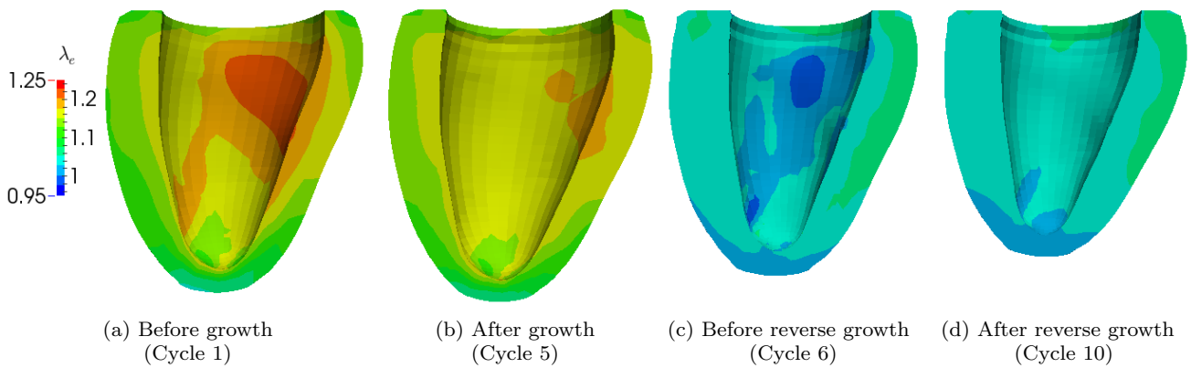
Fig. 10: Evolution of elastic myofiber stretch \lambda_e in the left ventricle as a result of growth and its reversal. Geometries are of the same scale.
