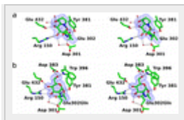
Figure 3. Stereo views (divergent “wall-eyed” stereo) of the ScHEX 6-Ac-Cas and E302Q ScHEX NAG–oxazoline active-site complexes. F_o-F_c omit electron density maps (with phases calculated prior to any modeling or refinement of any ligand) of each complex are shown in blue, contoured at 3.0 \sigma . (A) ScHEX 6-Ac-Cas complex (molecule A). (B) E302Q ScHEX NAG–oxazoline complex. Hydrogen bonds \leq 3.2 \text{ \AA} are shown as dashed lines. This figure was drawn with CCP4mg.
