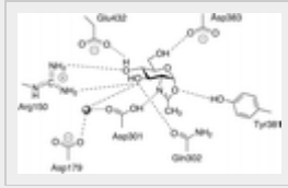
Scheme 2. Schematic Diagram of the Interactions between ScHEX and the Intermediate Oxazoline Trapped on the E302Q Variant a
