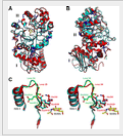
Figure 1. Structural comparison between SpHEX and ScHEX . (A) Front-view overlay of wild-type SpHEX (PDB entry 1HP5, red) with wild-type ScHEX (PDB entry 4C7D, cyan). The position of the active site is defined by the presence of NAG–thiazoline bound within the SpHEX binding pocket (NGT, yellow). The \beta/\alpha topology domain I and (\beta/\alpha)_8 barrel domain II are identified by roman numerals. Residues of the (\beta/\alpha)_8 barrel comprising catalytic domain II that differ in sequence between SpHEX and ScHEX are shown in ball-and-stick representation in ScHEX (blue). (B) Side-view of the complex (90° counter clockwise rotation about the y -axis relative to (A)). (C) Stereo view of SpHEX (PDB entry 1M01, red) and ScHEX (cyan/green) showing two alternate conformations adopted by loop 3 in ScHEX . Positions of the modeled loop 3 conformations A (0.7 occupancy) and B (0.3 occupancy) are shown in green and red, respectively. The loop 3B conformation corresponds to the active orientation of catalytic residues Asp301B and Glu302B (cyan in ScHEX and red in SpHEX ), which are ideally positioned to hydrogen bond with glycans in the active-site pocket. Residues Asp301A and Glu302A in conformation A are shown in green. The N -acetylglucosamine (GlcNAc) product complexed to SpHEX is shown in yellow. This figure was drawn with MacPyMOL 1.3.
