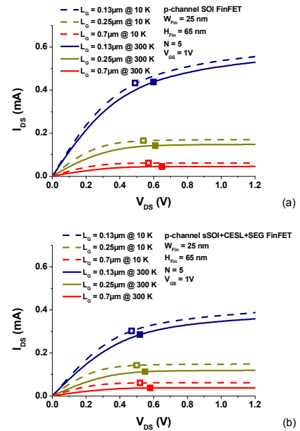
Fig. 1. Typical output characteristics I_D(V_{DS}) for standard a) and strained (b) p-channel FinFETs at 10 K and 300 K for various gate lengths. The square points represent the extracted I_{Dsat} and V_{Dsat} levels.
