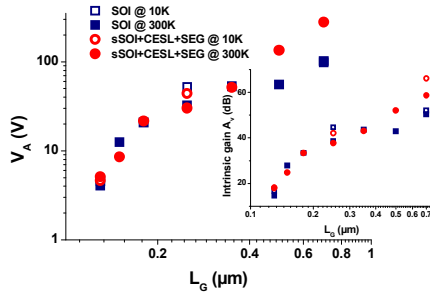
Fig. 4. The Early voltage V_{EA} versus the mask gate length; in the inset are represented the intrinsic gain A_V versus the mask gate length.
