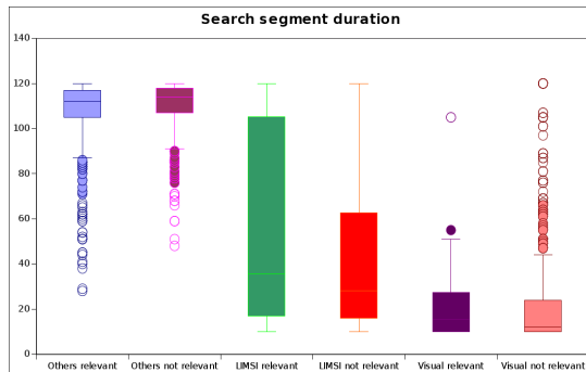
Figure 1: Boxplots showing segment duration variation proposed by others participants and our systems (i.e., LIMSIs and Visual)
