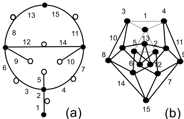
Figure 2. The dessin d'enfant (a) arising from the first subgroup of index 15 of the Kleinian group K^{(4)} and the line graph of the Petersen graph (b) that it stabilizes. The list of coset representatives corresponding to the labelling \{1, 2, \dots, 15\} is as follows [e, y, yx, yx^{-1}, yx^2, yxy, yx^{-1}y, (yx)^2, yxyx^{-1}, yx^{-1}yx, (yx^{-1})^2, yxyx^2, yxyx^{-1}y, yx^{-1}yx^2, yx^{-1}yxy] . Only the thin triangles (passing through e ) have their cosets mutually commuting.
