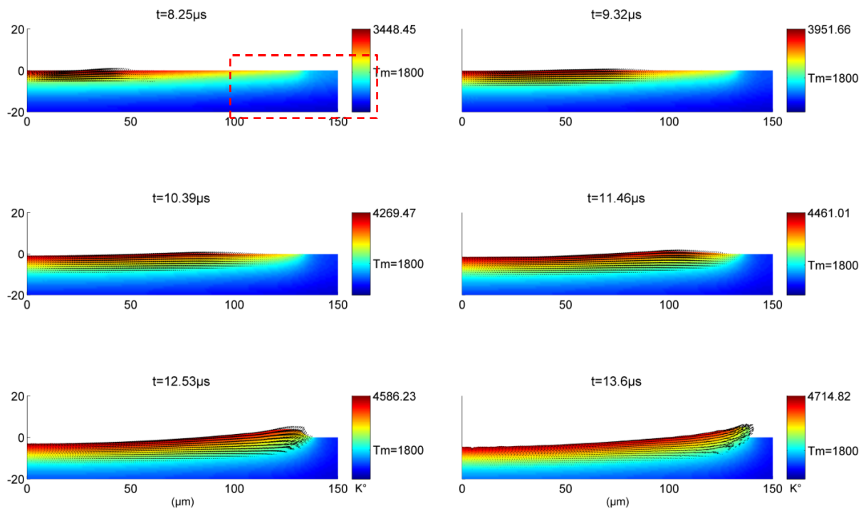
Figure 5: Temperature field ( K^\circ ), Arrows: liquid velocity
