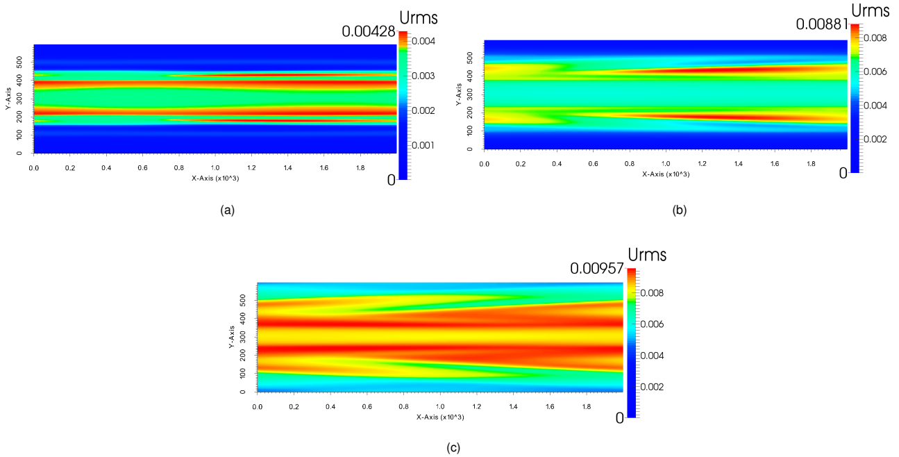
Figure 6: 2D U_{rms} fields for H20 (a), H20CD2P3 (b) and H50 (c) after 11.5 days of dynamics.
