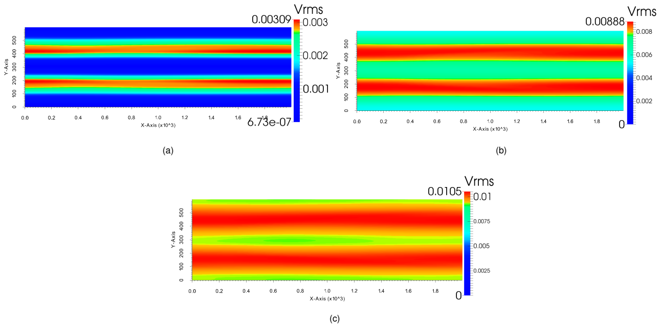
Figure 7: 2D V_{\text{rms}} fields for H20 (a), H20CD2P3 (b) and H50 (c) after 11.5 days of dynamics.
