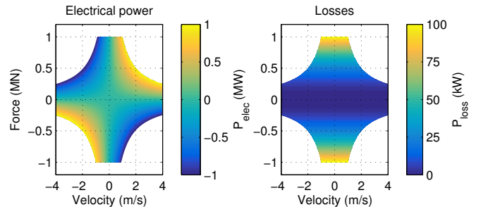
Fig. 3. Electrical power and electrical loss power as a function of Buoy velocity \dot{z} and Power Take-Off force f_{PTO} with F_{max} = 1 \text{ MN} , P_{max} = 1 \text{ MW} and c_{loss} = 0.1 \text{ MW/MN}^2
