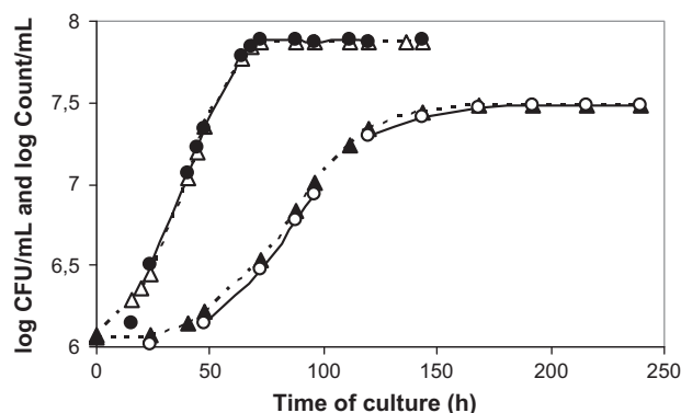
Fig. 1. O. oeni counts in FT80 broth at pH 5 (Δ): plate count; (•): FCM; pH 3.2 (▲) plate count, (○): FCM. The maximum standard deviations for these measurements were 0.073 for plate counts and 0.045 for FCM counts. The error tool bars were removed to make the graph clearer.
