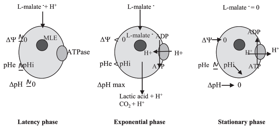
Fig. 7. Changes in force proton motive components and functioning of ATPase during MLF. At the beginning of the growth, \Delta\Psi was low and pH_{in} was equal to pH_{ex} ( \Delta pH \approx 0 ). During the growth of O. oeni , \Delta\Psi increases when malate enters the cells, the malolactic enzyme cleaves malic acid, and lactic acid and CO 2 are co-excreted with protons, which causes the pH_{in} to increase. This \Delta pH allows the entry of protons and the increase of the proton motive force with the synthesis of ATP by ATP synthase. When malic acid is totally exhausted, pH_{in} and \Delta\Psi decrease.
