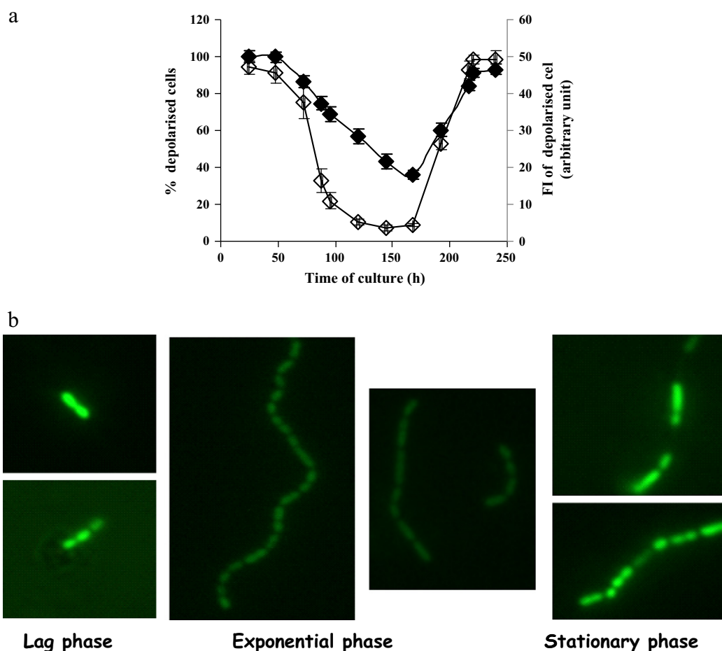
Fig. 2. Change in O. oeni cell depolarisation during MLF in FT80, pH 3.2. a: Percentage of depolarised cells (◇) and depolarisation level (FI) (◆) after DiBAC staining. The percentage of depolarised cells decreased up to 168 h (maximum polarisation). b: Photograph of O. oeni cells during MLF after DiBAC staining. The fluorescence intensity of cells after DiBAC staining was lower in the exponential phase than in the lag phase or at the end of the stationary phase.
