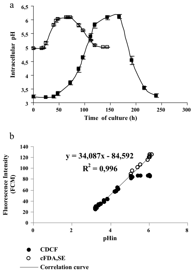
Fig. 3. a: Change in \text{pH}_{\text{in}} during MLF in FT80 medium, pH 3.2 (■), and FT80 medium, pH 5 (□). At the beginning and at the end of MLF, \text{pH}_{\text{in}} is equal to \text{pH}_{\text{ex}} . \text{pH}_{\text{in}} increased to 6.1 during growth. b: Calibration curve with CDCF and CFDA SE.
