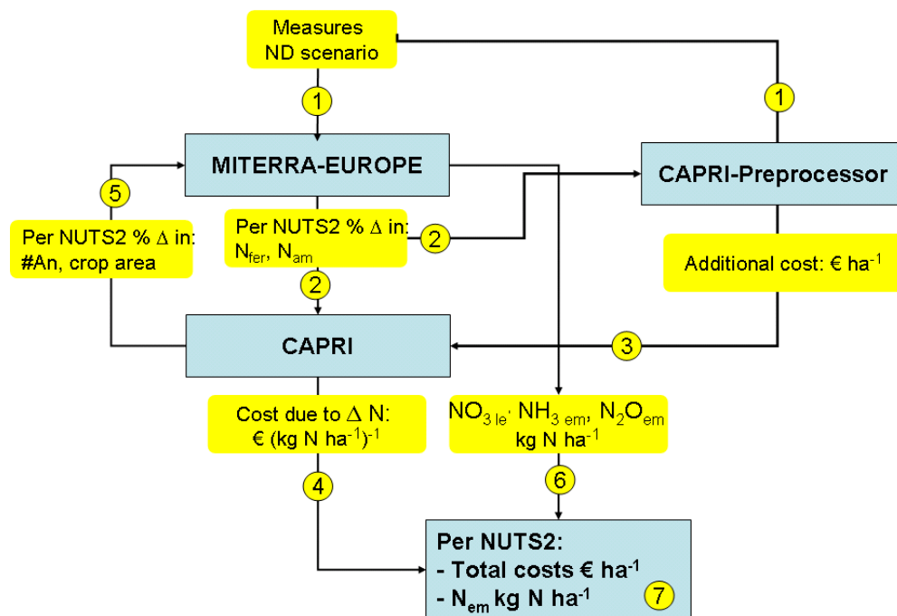
Figure 1. Coupling of MITERRA and CAPRI to assess the effects of the N-Directive.
