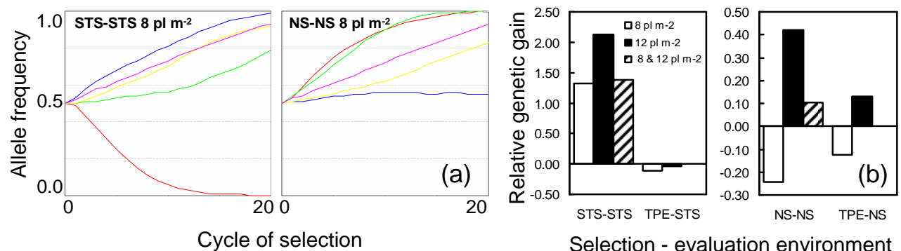
Figure 1 Mean changes in gene frequencies for +alleles associated with RA (--), LA (--), ME (--), CA (--) and SP (--) (a) and relative genetic gains for a set of selection experiments (b). Selection simulated for specific (8 or 12 pl m -2 ) and non-specific management (8 and 12 pl m -2 ) and STS, NS and TPE environments. For each management practice, genetic gains were evaluated in environments STS and NS. TPE-STS denote for selection in TPE environments and evaluation in STS environment type.
