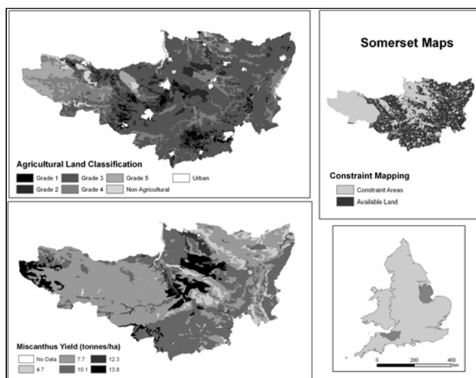
Figure 1: Yield distributions with and without soil quality constraints (AWC) and maps of ALC, yield and constraints in Somerset
