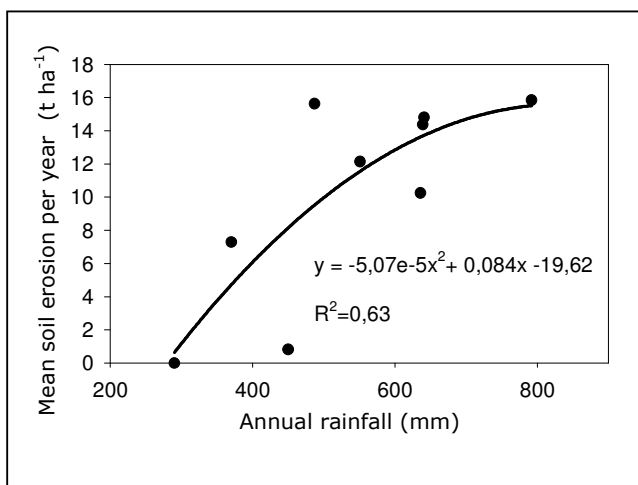
Fig. 1 – Relation between annual rainfall (from August to June) and soil erosion per year in the average of the studied cropping systems.
