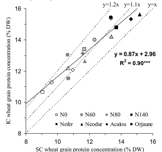
Figure 2: Wheat grain protein concentration in intercrop (IC) as a function of that in sole crop (SC) for the different N treatments and cultivars. Mean (n = 3)
