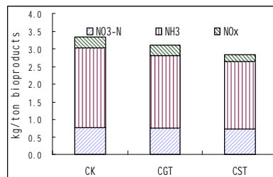
Fig. 1. Eutrophication ( \text{kgPO}_4\cdot\text{t}^{-1} bioproductivity) of different planting patterns
