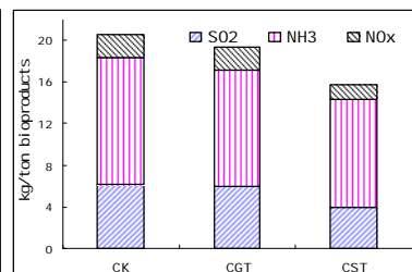
Fig. 2. Acidification ( \text{kgSO}_2\cdot\text{t}^{-1} bioproductivity) of different planting patterns
